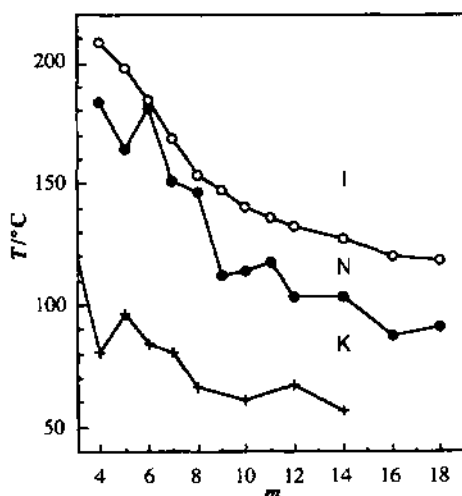
Fig. 3. Phase pattern diagram for series Cu1-1. m . Melting points (+) of bis[ N -( n -alkyl)salicylidiminato]copper(II) complexes [20] are also plotted for comparison.
