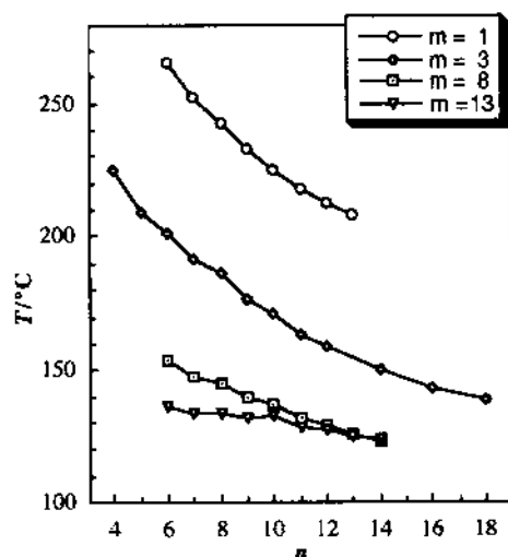
Fig. 5. Comparison of T_{\text{NI}} curves for series \text{Cu1-n.1} , \text{Cu1-n.3} , \text{Cu1-n.8} , and \text{Cu1-n.13} (adapted from Refs. [27,28,30]).
