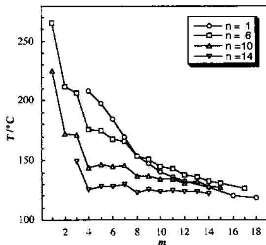
Fig. 6. Comparison of T_{NI} curves for series CuI-1.m , CuI-6.m , CuI-10.m , and CuI-14.m (adapted from Refs. [26,29,30]).
