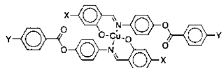
Fig. 2. Chemical modifications of the liquid-state archetypical complex to mesomorphic derivatives for metal-salicylaldehyde systems.
