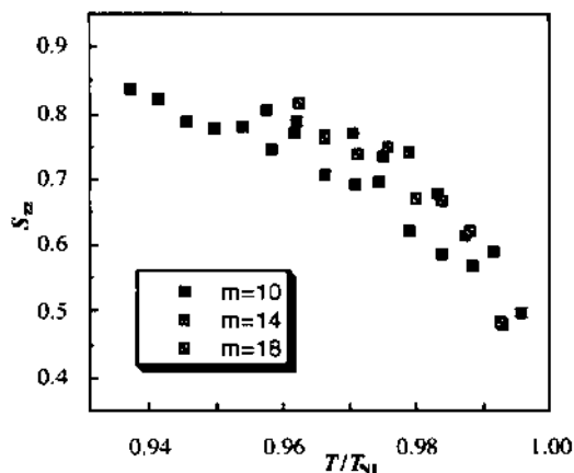
Fig. 8. Nematic orientational order parameter S_{zz} for selected homologues of \text{Ni1-1.}m determined by the ^1\text{H} NMR experiments. The molecular long axis ( z ) is defined as shown in the text.
