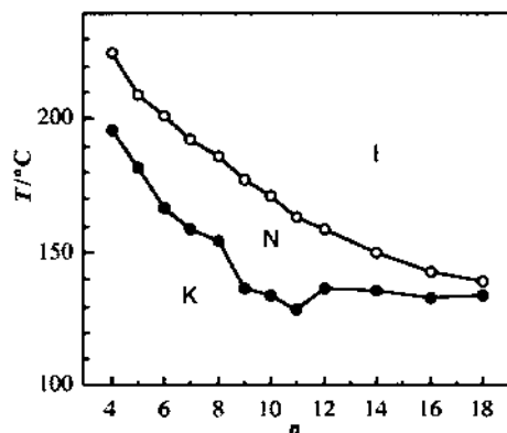
Fig. 4. Phase pattern diagram for series \text{Cu1-n.3} (adapted from Ref. [27]).
