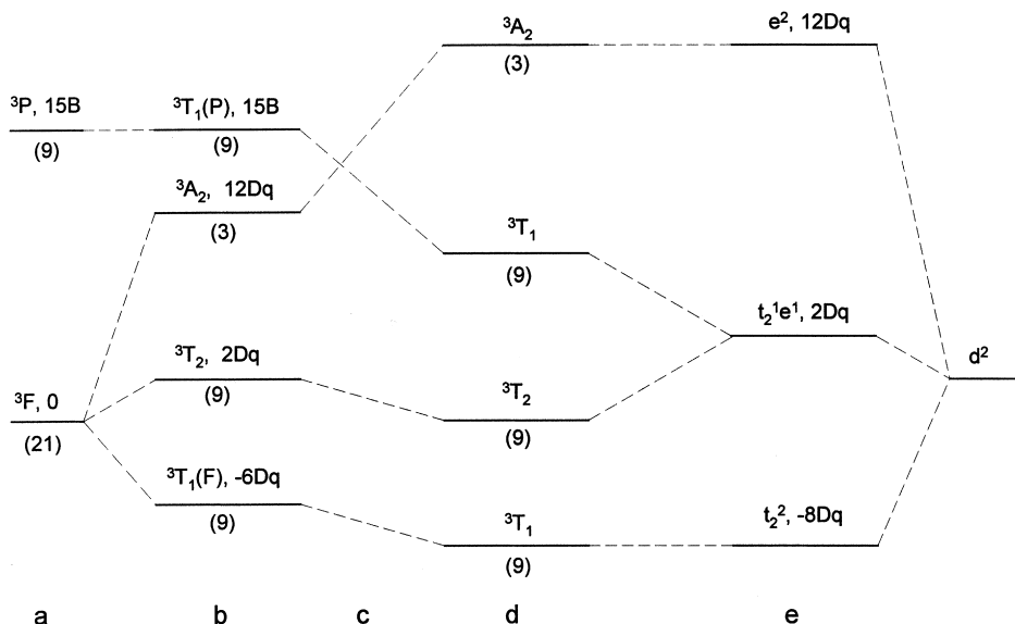
Fig. 24. Correlation diagram for the triplet terms of d^2 configuration in the octahedral crystal field: (a) free ion terms ( \hat{H}_0 includes \hat{V}^{ce} ); (b) weak field limit ( \hat{H}' = \hat{V}^{cf} ); (c) intermediate field ( \hat{H}' = \hat{V}^{ce} + \hat{V}^{cf} ); (d) strong field limit ( \hat{H}' = \hat{V}^{ce} ); (e) strong field configurations ( \hat{H}_0 includes \hat{V}^{ce} ).
