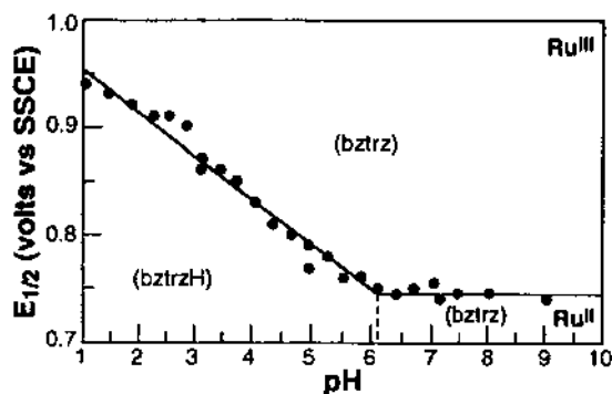
Fig. 12. pH-potential diagram for [(tpy)(bpy)Ru(bztrzH)]^{2+} (adapted from ref. [69]).
