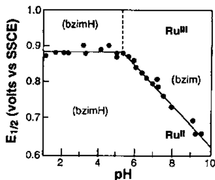
Fig. 11. pH-potential diagram for [(tpy)(bpy)Ru(bzimH)]^{2+} (adapted from ref. [69]).
