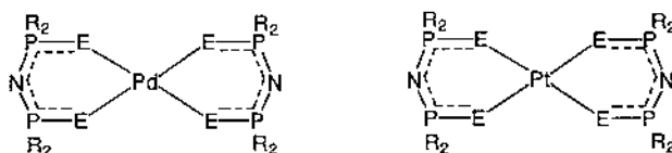
Fig. 17. The structures of [\text{Pd}(\text{PhO})_2(\text{S})\text{PNP}(\text{S})(\text{OPh})_2] [41], [\text{M}\{(\text{Pr}_2(\text{S})\text{P})_2\text{N}\}_2] ( \text{M} = \text{Pd} or \text{Pt} ) (D. Cupertino, R. Keyte, A.M.Z. Slawin, D.J. Williams, J.D. Woollins, unpublished work) and [\text{Pd}(\text{Ph}_2(\text{O})\text{PNP}(\text{Se})\text{Ph}_2)_2] ( \text{R} = \text{Ph} or \text{Pr} ) [40].
