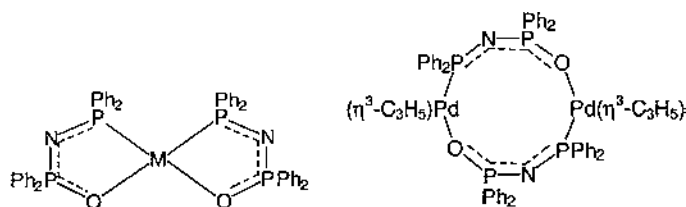
Fig. 2. The structures of \text{cis-}[M(\text{Ph}_2\text{P}(\text{O})\text{NPh}_2)_2] and [\text{Pd}(\eta^3\text{-C}_3\text{H}_5)(\text{Ph}_2\text{PNP}(\text{O})\text{Ph}_2)]_2 [12].
