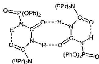
Fig. 34. The structure of [(\text{PhO})_2\text{P}(\text{O})\text{NHC}(\text{O})\text{NHC}(\text{O})\text{N}(\text{nPr})_2] [86].
