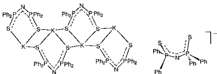
Fig. 7. The structures of \text{K}[\text{N}(\text{P}(\text{S})\text{Ph}_2)_2] [17] and [\text{K}(18\text{-crown-6})]^+ [\text{N}(\text{P}(\text{S})\text{Ph}_2)_2]^- [18].
