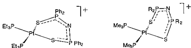
Fig. 18. The structures of [\text{Pt}\{\text{N}(\text{P}(\text{S})\text{Ph}_2)_2\}_2(\text{PEt}_3)_2]^+ and [\text{Pt}\{(\text{PhO})_2(\text{S})\text{PNP}(\text{S})(\text{OPh})_2(\text{PMe}_3)_2\}]^+ [43].
