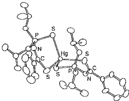
Fig. 43. Molecular structure of [Hg(PhC(S)NP(S)(O i Pr) 2 )] [90].
