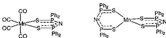
Fig. 12. The structures of [\text{Mn}(\text{CO})_4\{(\text{Ph}_2(\text{S})\text{P})_2\text{N}\}] [27] and [\text{Mn}\{(\text{Ph}_2(\text{S})\text{P})_2\text{N}\}_2] [28].
