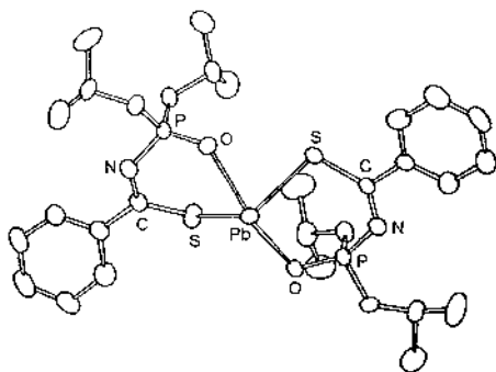
Fig. 44. Molecular structure of [\text{Pb}\{\text{PhC}(\text{S})\text{NP}(\text{O})(\text{O}^i\text{Pr})_2\}_2] [72].
