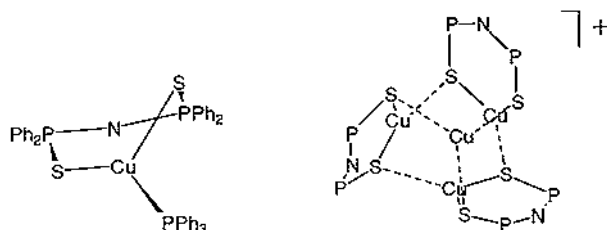
Fig. 19. The structures of [\text{Cu}(\text{PPh}_3)\{(\text{Ph}_2(\text{S})\text{P})_2\text{N}\}] [44] and [\text{Cu}_4\{(\text{Ph}_2(\text{S})\text{P})_2\text{N}\}_3]^+ [\text{CuCl}_2]^- (with phenyls omitted for clarity) [45].
