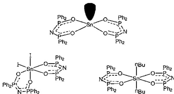
Fig. 23. The structures of [\text{Sn}(\text{Ph}_2(\text{O})\text{P})_2\text{N}]_2 , [\text{SnI}_2\{(\text{Ph}_2(\text{O})\text{P})_2\text{N}\}_2] [49] and [\text{Sn}(\text{}^n\text{Bu})_2\{(\text{Ph}_2(\text{O})\text{P})_2\text{N}\}_2] [50].
