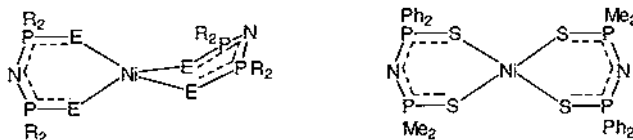
Fig. 16. The structures of [\text{Ni}((\text{Ph}_2(\text{S})\text{P})_2\text{N})_2] [6,34,35], [\text{Ni}((\text{Me}_2(\text{S})\text{P})_2\text{N})_2] [36,37], [\text{Ni}(\text{Pr}_2(\text{S})\text{P})_2\text{N}]_2 [38] and [\text{Ni}(\text{Ph}_2(\text{S})\text{PNP}(\text{S})\text{Me}_2)_2] [39].
