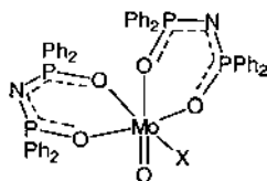
Fig. 10. The structure of [\text{MoX}(\text{O})\{(\text{Ph}_2(\text{O})\text{P})_2\text{N}\}_2] (X = Cl or O) [25].
