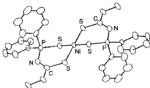
Fig. 39. Molecular structure of [\text{Ni}\{\text{MeHNC}(\text{S})\text{NP}(\text{S})\text{Ph}_2\}_2] [88].
