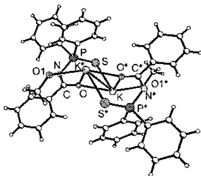
Fig. 38. Molecular structure of K[PhC(O)NP(S)Ph 2 ] 2 · 2CH 3 OH [70].
