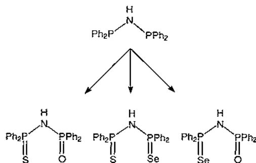
Scheme 2. Unidentate complexes of [\text{Ph}_2(\text{O})\text{PNHPPPh}_2] with Rh, Ir, Pd, Pt and Au [9–11].
