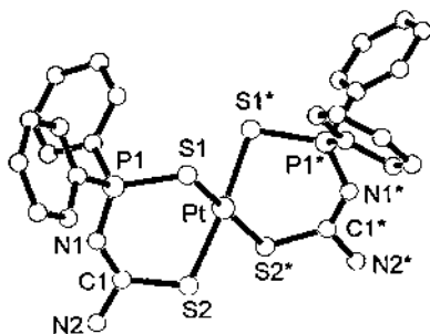
Fig. 41. Molecular structure of [\text{Pt}\{\text{H}_2\text{NC}(\text{S})\text{NP}(\text{S})\text{Ph}_2\}_2] \cdot (\text{Et}_2\text{O}) [70].
