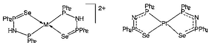
Fig. 4. The structures of [\text{Pt}(\text{Ph}_2\text{P}(\text{Se})\text{NHPPH}_2)_2]\text{Cl}_2 and [\text{Pt}(\text{Ph}_2\text{P}(\text{Se})\text{NPPH}_2)_2] [14].
