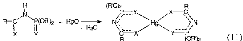
Fig. 43. Molecular structure of [Hg(PhC(S)NP(S)(O i Pr) 2 )] [90].
