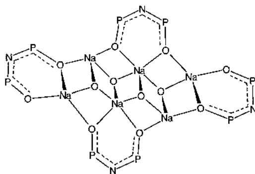
Fig. 5. The structure of \text{Na}[(\text{PhO})_2(\text{O})\text{PNP}(\text{O})(\text{OPh})_2] with two bridging chelates at the front, and the back omitted for clarity [15].
