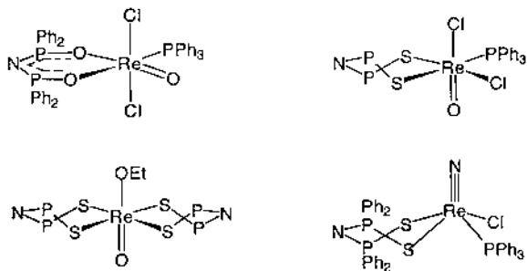
Fig. 13. The structures of [\text{Re}(\text{O})\text{Cl}_2\{(\text{Ph}_2(\text{O})\text{P})_2\text{N}\}(\text{PPh}_3)] , [\text{Re}(\text{O})\text{Cl}_2\{(\text{Ph}_2(\text{S})\text{P})_2\text{N}\}(\text{PPh}_3)] , [\text{ReO}(\text{OEt})\{(\text{Ph}_2(\text{S})\text{P})_2\text{N}\}_2] [29] and [\text{Re}(\text{N})\text{Cl}\{(\text{Ph}_2(\text{S})\text{P})_2\text{N}\}(\text{PPh}_3)] [30].
