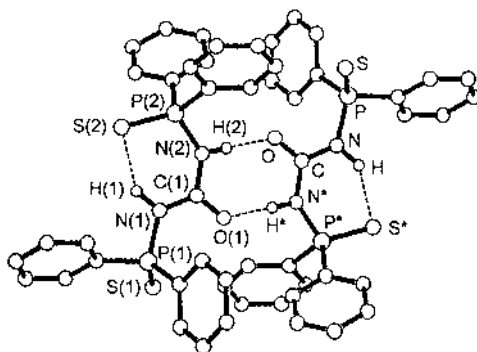
Fig. 35. The structure of [\text{Ph}_2(\text{S})\text{PNHC}(\text{O})\text{NHP}(\text{S})\text{Ph}_2] [87].
