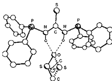
Fig. 36. Molecular structure of [\text{Ph}_2\text{PNHC}(\text{S})\text{NHPPh}_2] \cdot \text{Me}_2\text{SO} [87].
