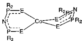
Fig. 15. The structures of [\text{Co}((\text{Me}_2(\text{S})\text{P})_2\text{N})_2] and [\text{Co}((\text{Ph}_2(\text{Se})\text{P})_2\text{N})_2] [33].
