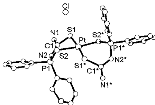
Fig. 40. Molecular structure of [\text{Pt}\{\text{H}_2\text{NC}(\text{S})\text{NP}(\text{S})\text{Ph}_2\}(\text{H}_2\text{NC}(\text{S})\text{NHP}(\text{S})\text{Ph}_2)]^+ \text{Cl}^- [70].
