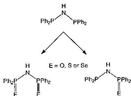
Scheme 1. Heteroatom ligands derived from DPPA.
