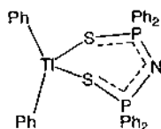
Fig. 22. The structure of [\text{TiPh}_2\{(\text{Ph}_2(\text{S})\text{P})_2\text{N}\}] [48].
