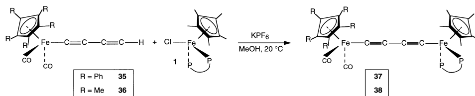
Scheme 15.
