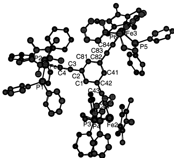
Fig. 11. Crystal structure of 31 . Selected bond distances (Å) and angles (deg); Fe1–P1, 2.178(3); Fe1–P2, 2.166(3); Fe2–P3, 2.161(3); Fe3–P4, 2.168(3); Fe3–P5, 2.181(4); Fe3–P6, 2.170(3); Fe1–Cp* (Centroid1) , 1.750; Fe2–Cp* (Centroid2) , 1.742; Fe3–Cp* (Centroid3) , 1.738; Fe1–C4, 1.90(1); Fe2–C44, 1.89(1); Fe3–C84, 1.92(1); Fe1–Fe2 (Intra) , 10.05; Fe1–Fe3 (Intra) , 10.48; Fe2–Fe3 (Intra) , 10.32; C3–C4, 1.24(2); C43–C44, 1.23(2); C83–C84, 1.21(1); C1–C2, 1.38; C2–C81, 1.39(1); C81–C82, 1.41(1); C41–C82, 1.38(2); C41–C42, 1.39(1); C1–C2, 1.41(1); P1–Fe1–P2, 84.7(1); P3–Fe2–P4, 85.7(1); P5–Fe3–P6, 85.9(1); P1–Fe1–C4, 84.8(3); P2–Fe1–C4, 84.8(3); P3–Fe2–C44, 83.7(2); P4–Fe2–C44, 83.5(3); P5–Fe3–C84, 84.1(4); P6–Fe3–C84, 83.7(4); Fe1–C4–C3, 178(1); Fe2–C44–C43, 177.4(9); Fe3–C84–C83, 178.4(8); C4–C3–C2, 173(1); C4–C43–C42, 177.0(1); C84–C83–C22, 175.5(9).
