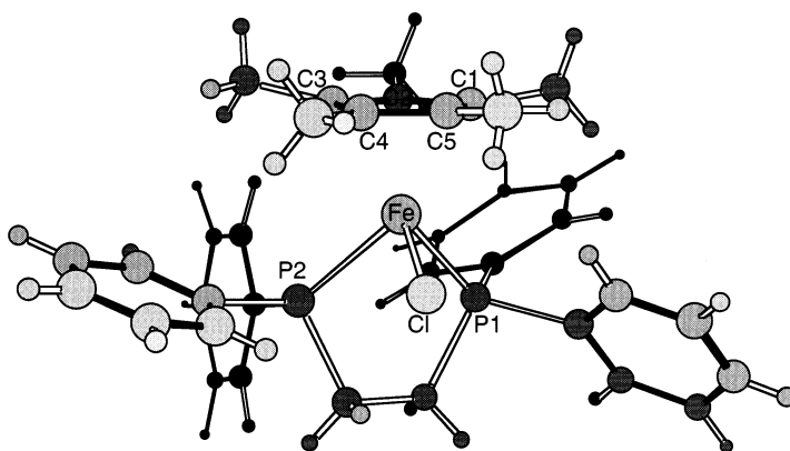
Fig. 7. Crystal structure of the iron(III) chloro complex [353].
