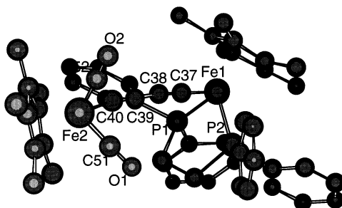
Fig. 10. Crystal structure of 38 . Selected bond distances (Å) and angles (deg): Fe1–P1, 2.190(3); Fe1–P2, 2.172(3); Fe1–C37, 1.886(9); Fe2–C51, 1.76(1); Fe2–C52, 1.73(1); Fe2–C40, 1.90(1); Fe1–Cp* (Centroid1) , 1.740(3); Fe2–Cp* (Centroid2) , 1.706(3); Fe1–Fe2 (Intra) , 7.57; C37–C38, 1.21(1); C38–C39, 1.36(1); C39–C40, 1.24(1); C51–O1, 1.13(1); C52–O2, 1.15(2); P1–Fe1–P2, 85.7(1); P2–Fe1–C37, 83.4(3); P1–Fe1–C37, 83.8(3); Fe1–C37–C38, 177.8(8); C51–Fe2–C52, 95.3(5); C52–Fe2–C40, 90.4(5); C51–Fe2–C40, 87.3(5); Fe2–C40–C39, 172.0(1); Fe2–C51–O1, 176(1); Fe2–C52–O2, 178.0(1); C37–C38–C39, 175(1); C40–C39–C38, 178.4(9).
