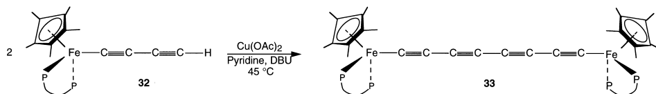
Scheme 13.
