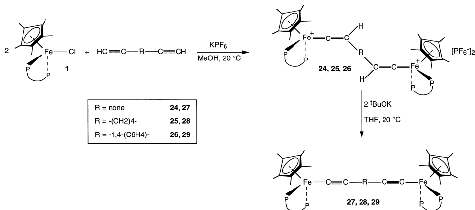
Scheme 9.
