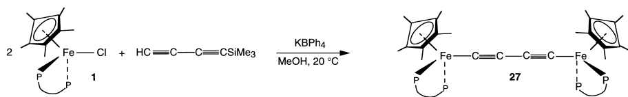
Scheme 10.
