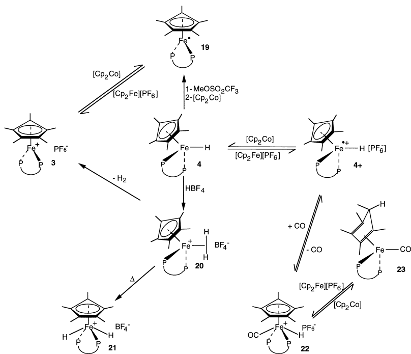
Scheme 8.
