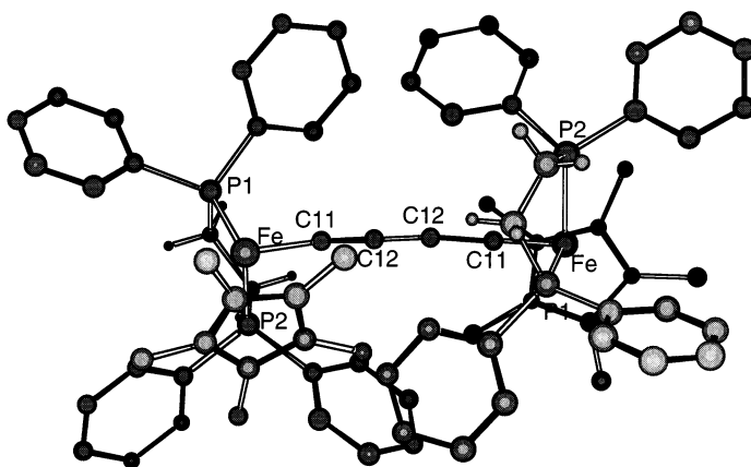
Fig. 8. Crystal structure of 27^+ . Selected bond distances (Å) and angles (deg): Fe–P1, 2.238(2); Fe–P2, 2.206(2); Fe–C11, 1.830(8); Fe–Cp centroid , 1.766; Fe–Fe (intra) , 7.43; C11–C12, 1.236(9); C12–C12, 1.36(1); P1–Fe–P2, 84.65(8); P2–Fe–C11, 84.4(2); P1–Fe–C11, 93.4(2); Fe–C11–C12, 167.0(6); C11–C12–C12, 177(1).
