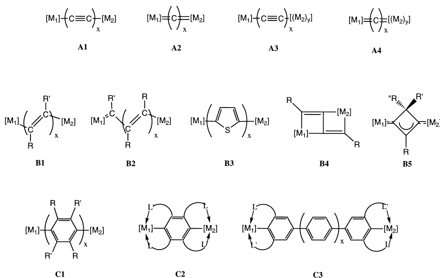
Fig. 5. Known type III-3-bridged dinuclear organometallics with polyethyne-diyl-, polyethene-diyl- and para-polyphenylene-based regular bridges.
