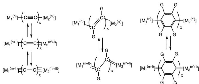
Fig. 4. Possible mesomeric structures for polyethyne-diyl-, polyethene-diyl- and para -polyphenylene-based bridges in dinuclear type III-3 organometallic complexes.
