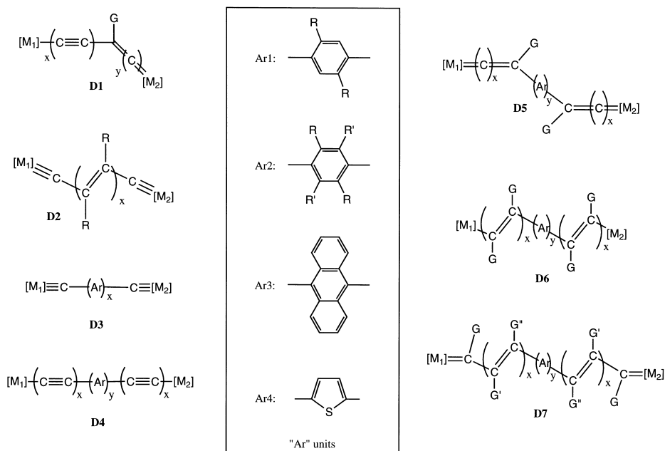
Fig. 6. Known type III-3-bridged dinuclear organometallics with mixed sp or sp 2 carbon-based units in the bridge.
