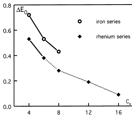
Fig. 9. Comparative evolution of the oxidation potential difference \Delta E^0 upon chain increase in the di-iron (○) and di-rhenium series (◆). The dashed line indicate irreversible redox events in CV.
