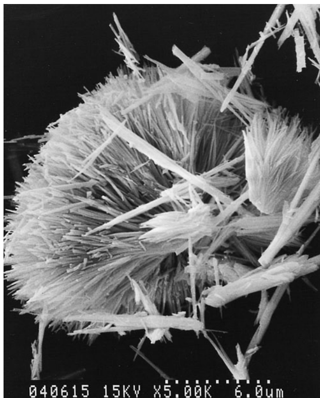
Fig. 6. SEM picture of \text{K}_2\text{Ni}_4(\text{P}_2\text{O}_7)_2(\text{PO}_4) prepared in molten \text{KNO}_3 at 773 K.
