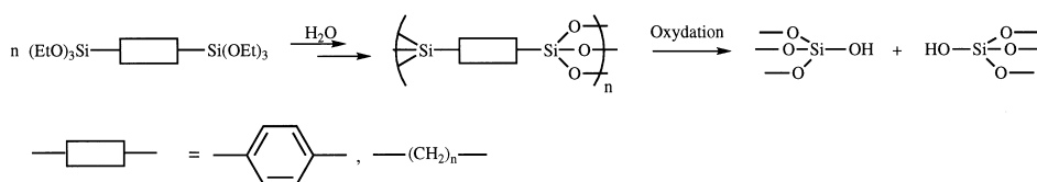
Scheme 6. Oxidative elimination of organic templates in poly(silsesquioxanes) [37].
