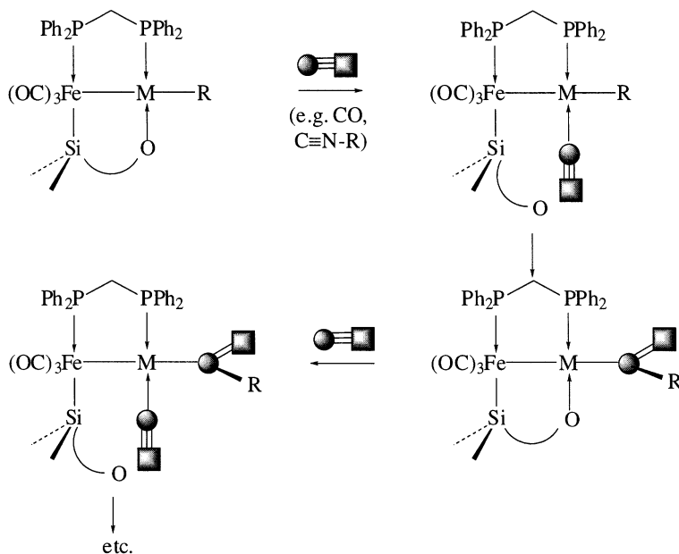
Scheme 1. Substrate coordination/migratory insertion sequence resulting from the opening and bridging behaviour of the alkoxyisilyl ligand (M = Pd, Pt).
