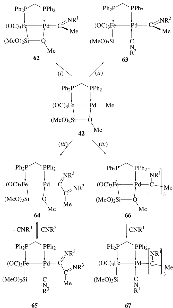
Scheme 3. Reactions in \text{CH}_2\text{Cl}_2 , -10 to 25^\circ\text{C} . (i) 1 equiv. \text{C}\equiv\text{NR}^1 [ \text{R}^1 = \text{C}_6\text{H}_4(\text{o-OMe}) ], (ii) 2 equiv. \text{C}\equiv\text{NR}^2 [ \text{R}^2 = \text{t-Bu} ], (iii) 2 equiv. \text{C}\equiv\text{NR}^3 [ \text{R}^3 = \text{C}_6\text{H}_3\text{Me}_2\text{-2,6} ], (iv) 3 equiv. \text{C}\equiv\text{NR}^1 .
