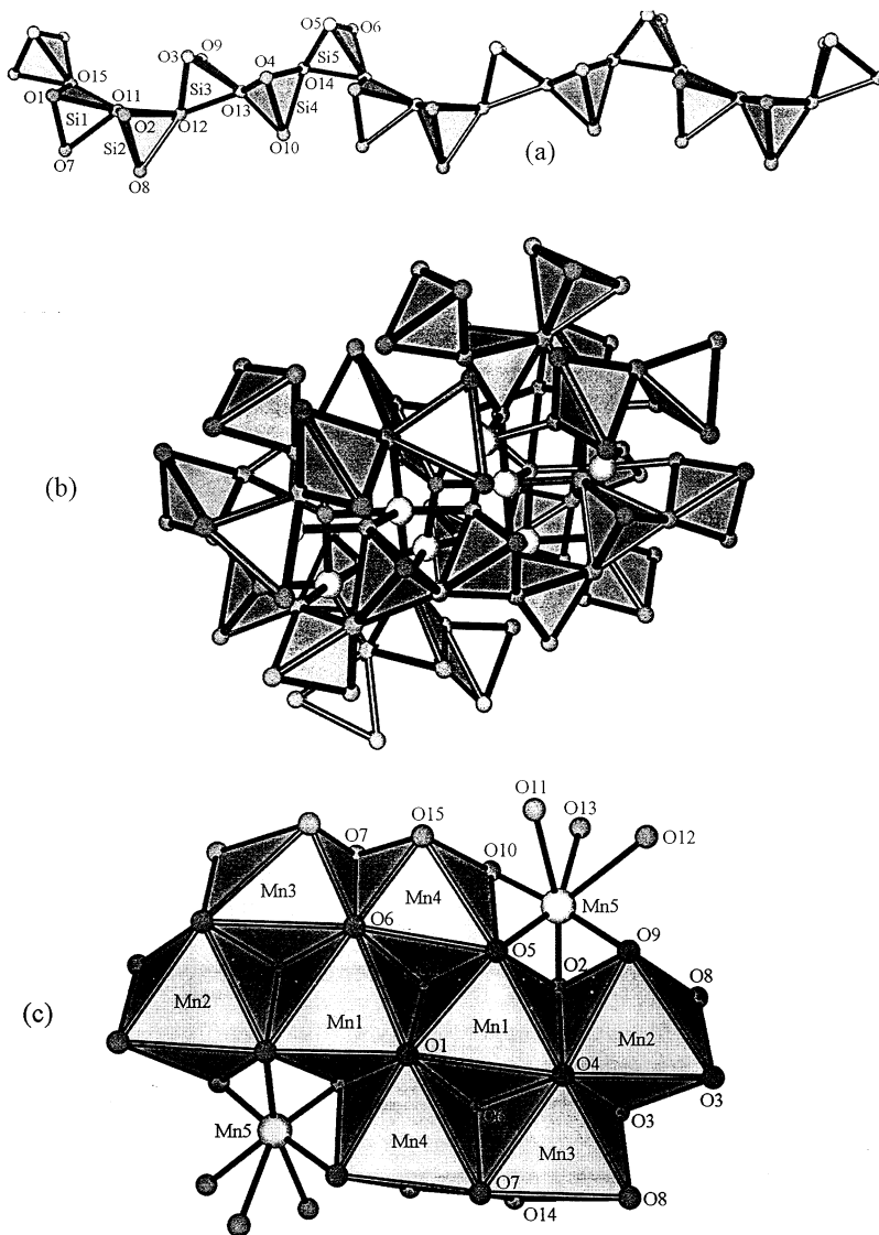
Fig. 6. Retrosynthesis of the crystal structure of rhodonite \text{MnSiO}_3 ( Z=20 ). (a) Linear chain of corner-sharing tetrahedra. (b) Model cluster [\text{MnSi}_3\text{O}_{10}]^{60-} extracted from the rhodonite network. (c) Manganese-oxygen core of the model cluster evidencing the pivot atom Mn5.
