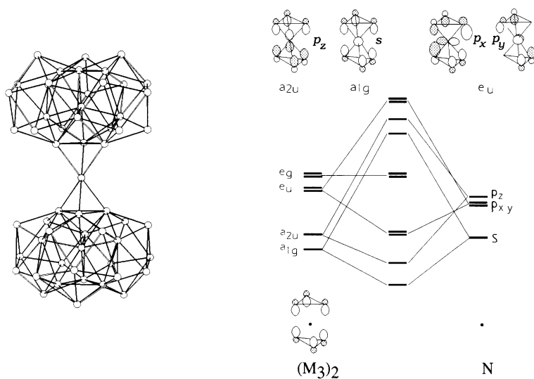
Fig. 22. Bonding scheme around the central N atom within the \text{M}_{28}\text{NM}_{28} cluster ( \text{D}_{3d} ).
