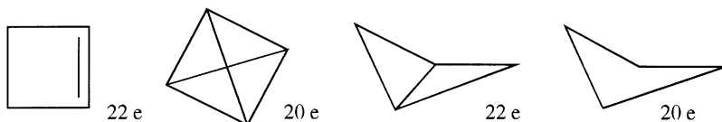
Fig. 13. Various geometrical configurations for \text{M}_4 species.
