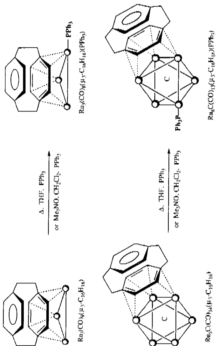
Scheme 7. Reaction of \text{Ru}_3(\text{CO})_9(\mu_3\text{-C}_{10}\text{H}_{16}) and \text{Ru}_6\text{C}(\text{CO})_{14}(\mu_3\text{-C}_{10}\text{H}_{16}) with triphenylphosphine.
