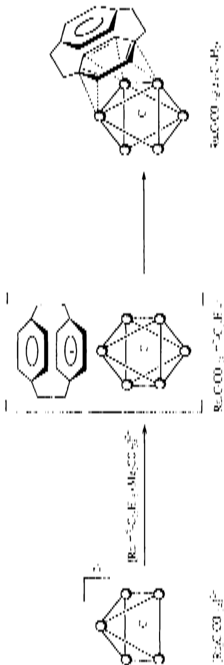
Scheme 11. Reaction of [\text{Ru}_5\text{C(CO)}_{14}]^{2-} with [\text{Ru}(\eta^6\text{-C}_{10}\text{H}_{16})(\text{MeCN})_3]^{2+} .
