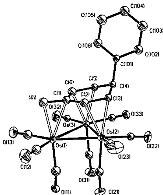
Fig. 3. X-ray structure of \text{Os}_3(\text{CO})_9(\mu_3\text{-}\eta^2\text{:}\eta^2\text{:}\eta^2\text{-NH-C}_6\text{H}_5\text{Ph}) . Reprinted with permission from Organometallics. Copyright 1997 American Chemical Society.
