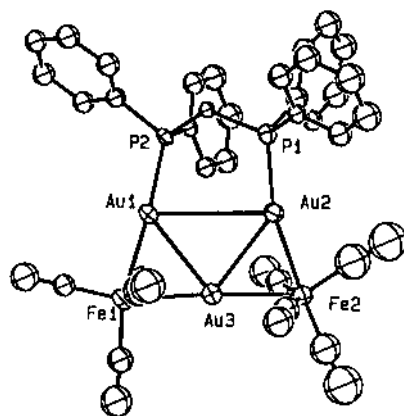
Fig. 20. X-ray structure of [\text{Au}_3\text{Fe}_2(\text{CO})_8(\text{dppm})]^- . Reprinted with permission from Organometallics. Copyright 1997 American Chemical Society.
