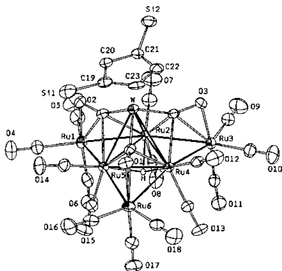
Fig. 22. X-ray structure of [\eta^5\text{-C}_5\text{H}_3(\text{TMS})_2]\text{WRu}_6(\mu_3\text{-H})(\text{CO})_{18} . Reprinted with permission from Journal of American Chemical Society. Copyright 1997 American Chemical Society.
