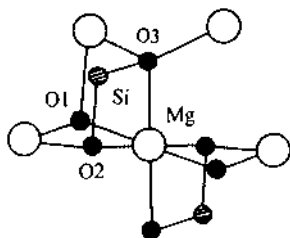
Fig. 12. The geometry of the C_i octahedron in \text{Mg}_2\text{SiO}_4 , depicting the bridging between the \text{SiO}_4 and \text{MgO}_6 polyhedra via common O2/O3 edges (Mg–O _i spacings: 2.09, 2.07, 2.13 Å for i = 1, 2 and 3, respectively [25]).
