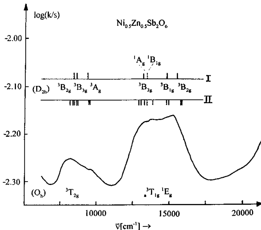
Fig. 18. Diffuse reflection spectra of the mixed crystal series \text{Zn}_{1-x}\text{Ni}_x\text{Sb}_2\text{O}_6 with x = 0.5 . Assignment ( D_{2h} symmetry, {}^3\text{B}_{1g} ground state; octahedral parent terms are also given) and fitting of band positions (dotted markings refer to the spin-forbidden transitions to {}^1\text{A}_g , {}^1\text{B}_{1g} ) with the parameter set of Eq. (11): I and II without and with LS coupling, respectively.
