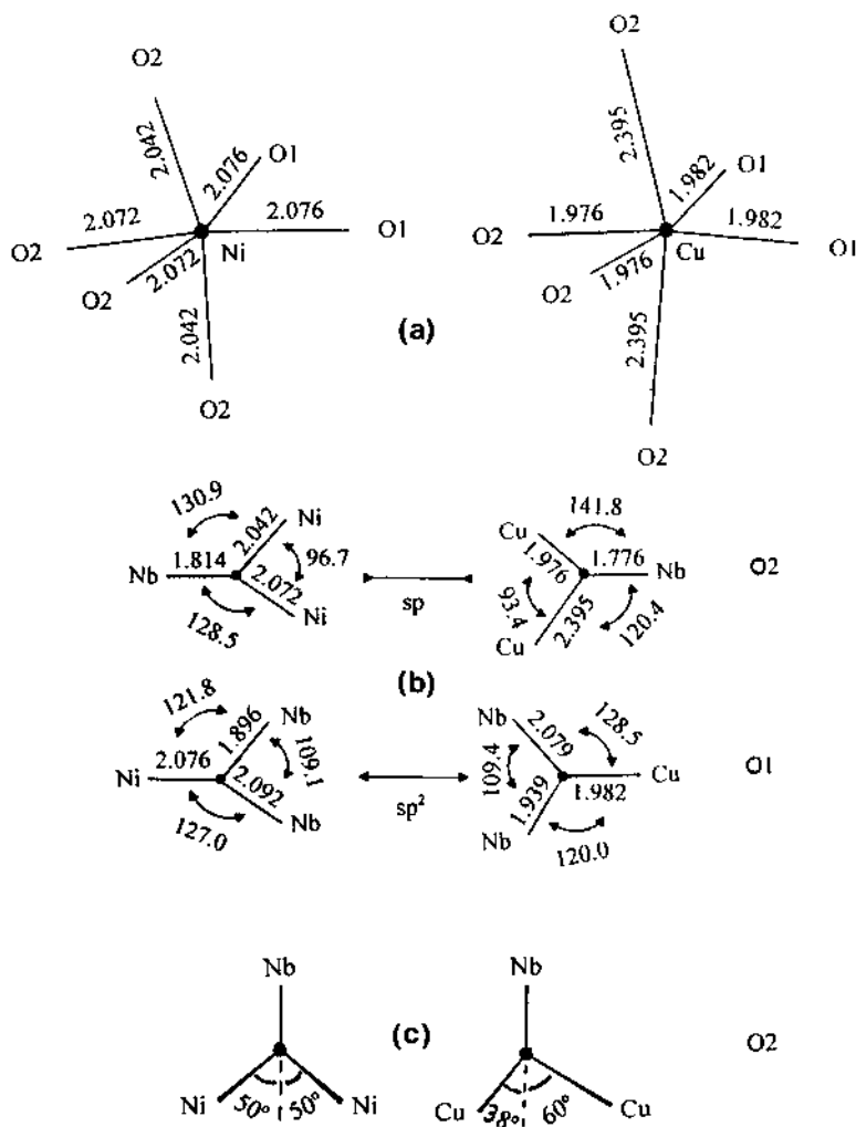
Fig. 27. The geometries of the \text{NiO}_6(\text{CuO}_6) polyhedra (a) and of the cationic coordination of the oxygen atoms O1 and O2 (only approximately planar) (b) in the orthorhombic columbites \text{NiNb}_2\text{O}_6(\text{CuNb}_2\text{O}_6) ; spacings (Å) and angles (°) from [43] ([44]). The angles between the \text{sp}_z lone pair on the O2 atoms and the two M-O2 bonds are \beta = 50.5(1.0)^\circ for Ni, but strongly diverging for Cu (c). The angle between the \text{sp}^2 hybrid orbital and the Ni(Cu)-O1 bond is 2.6(4.3)^\circ .
