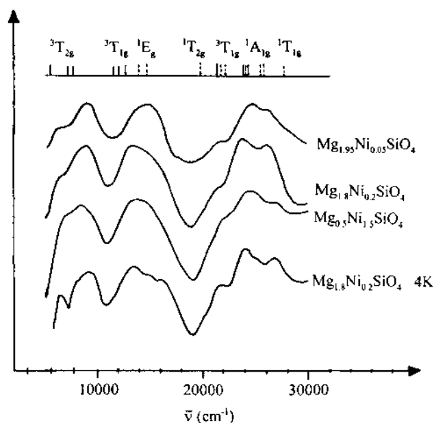
Fig. 13. d–d Reflection spectra (298 K) of \text{Ni}^{2+} on the octahedral C_s and C_i sites of \text{Mg}_2\text{SiO}_4 . The calculated energy positions are those due to \text{Ni}^{2+} on the \text{Mg}^{2+} site ( C_s ) in \text{LiMgPO}_4 (Fig. 7). The 4 K spectrum of \text{Mg}_{1.8}\text{Ni}_{0.2}\text{SiO}_4 in high resolution is shown below. The intensity corresponds to \log k/s for the 4 K and to reflectivity for the 298 K spectra.
