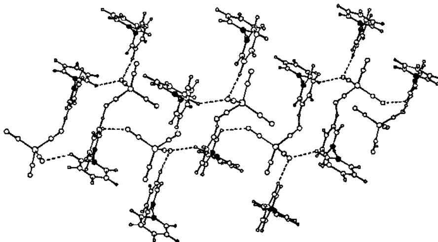
Fig. 19. C–H...O hydrogen bonding network in 8 (N atoms shaded).
