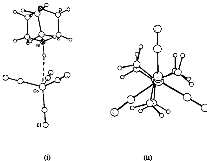
Fig. 7. Molecular structure of 4a . (i) The short cation–anion contact via the N–H···Co hydrogen bond from a perpendicular view. (ii) The staggered cation–anion conformation.
