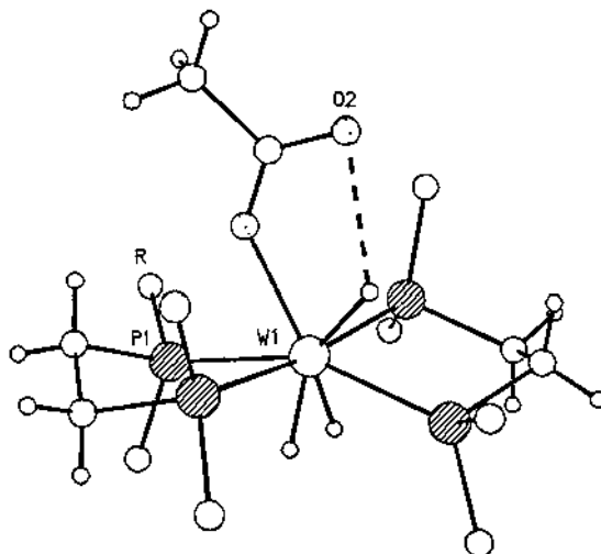
Fig. 3. Illustration of the W–H···O hydrogen bond in the compound [\text{WH}_3(\eta^1\text{-OCOMe})(\text{dppe})_2] {dppe, 1,2-bis(diphenylphosphinoethane)}. Drawn using coordinates from Ref. [13]b).
