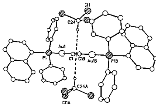
Fig. 6. C–H \cdots\pi interactions in an organometallic complex described in Ref. ([32]a), from which the atomic coordinates were also taken.
