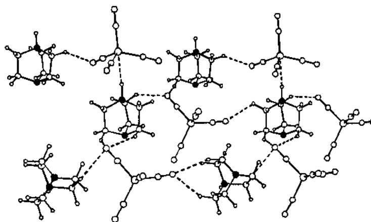
Fig. 16. C–H \cdots O hydrogen bonding network in 4a (N atoms shaded).
