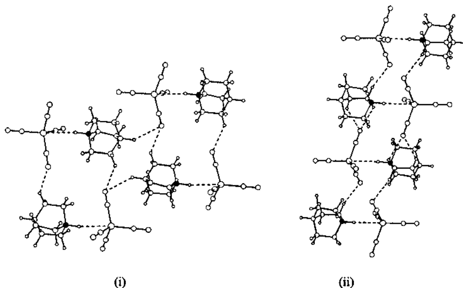
Fig. 15. C–H \cdots O hydrogen bond networks in 3 involving the carbonyl acceptor groups: (i) C(2)O(2), and (ii) C(3)O(3) and C(4)O(4) (N atoms are shaded).
