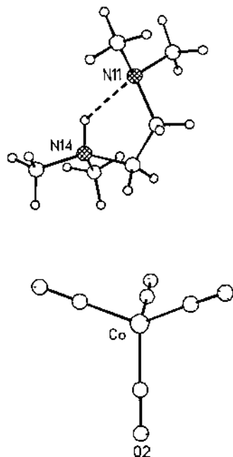
Fig. 9. Molecular structure of 6 , showing the intramolecular \text{N}-\text{H}^+\cdots\text{N} hydrogen bond. Coordinates taken from Ref. [37].
