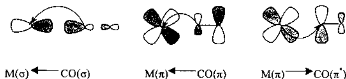
Fig. 4. Schematic representation of a molecular orbital (MO) description of the M–CO bonding interaction.
