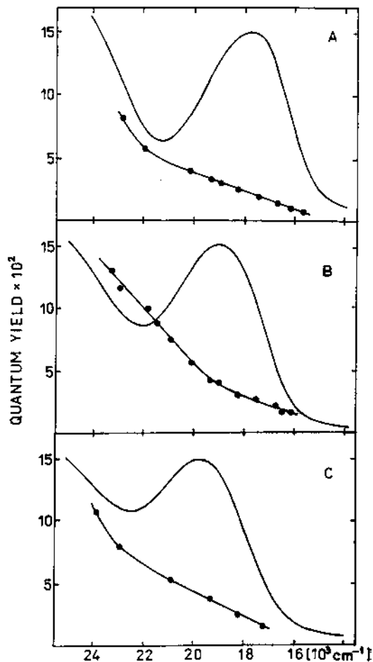
Fig. 3. Photochemical substitution of \text{Cr}(\text{CO})_4(\text{bpy}) by \text{PPh}_3 : Excitation energy dependence of the quantum yield and the absorption spectrum of \text{Cr}(\text{CO})_4(\text{bpy}) measured in various solvents [39]. (A) 6:1 (v:v) \text{C}_2\text{Cl}_4 : \text{C}_6\text{H}_6 mixture; (B) \text{C}_6\text{H}_6 ; (C) \text{CH}_2\text{Cl}_2
