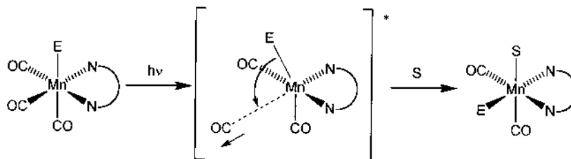
Fig. 6. Dissociative photochemical substitution/isomerisation of \text{Mn}(\text{E})(\text{CO})_3(\text{diimine}) complexes. Dissociation of the equatorial CO ligand is accompanied by a concerted movement of the axial ligand E into the equatorial plane. E = Cl, Br, I; diimine = bpy, 'Pr–PyCa or 'Pr–DAB. The solvent molecule S probably starts to coordinate to the axial position at later stages of the reaction. The primary photoproduct undergoes a back-reaction with CO, substitution of S by a stronger Lewis base, or a further photolysis to yield radicals [54–56]. A similar mechanism applies to the photochemistry of \text{Ru}(\text{I})(\text{Me})(\text{CO})_2(\text{bpy}') [91]
