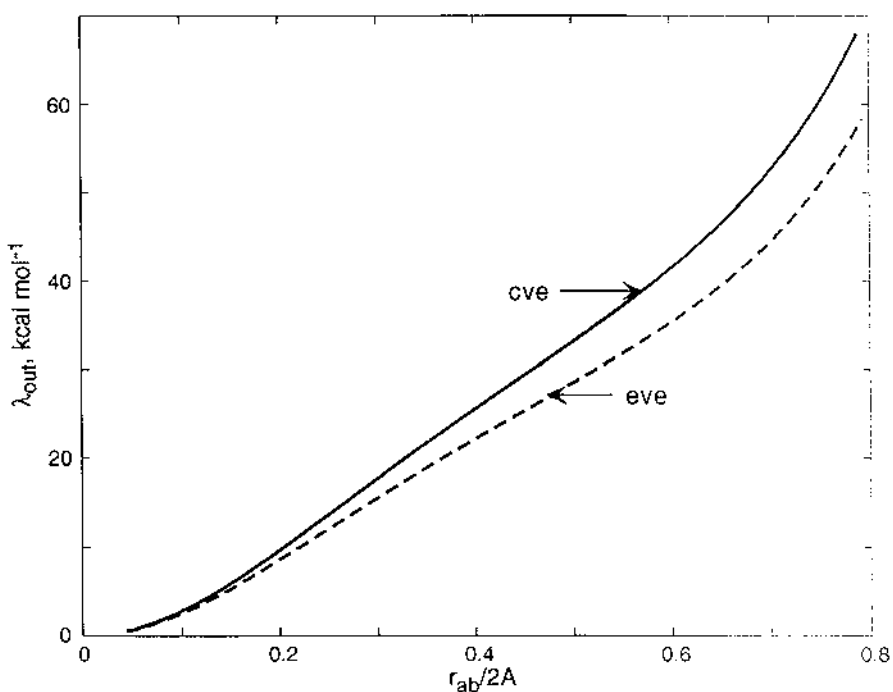
Fig. 4. Plot of the outer-shell reorganization energy \lambda_{\text{out}} versus r_{\text{ab}}/2A calculated using the ellipsoidal cavity model. The curves are constructed assuming that the charge transfer sites are located symmetrically a distance r_{\text{ab}} apart on the major axis of the ellipsoid: cve and eve represent the constant-volume ellipsoid and minimum-enclosing-volume ellipsoid models, respectively [39]. The cve assumption yields an ellipsoid with major axis ( 2A ), minor axes ( 2B ), and interfocal length ( R ) equal to 18.4, 7.10 and 17.0 \text{ \AA} , respectively, while the corresponding eve axes and interfocal length are 22.7, 8.42 , and 10.54 \text{ \AA} . The cve model constructs a cavity with a volume equal to that of [(\text{NH}_3)_5\text{Ru}^{\text{II}}-4,4'\text{-bpy}-\text{Ru}^{\text{III}}(\text{NH}_3)_3]^{5+} idealized as two spheres of effective radius 3.87 \text{ \AA} . The major axis of the ellipsoid just encloses the two axial amines which extend 3.55 \text{ \AA} from the metal centers. The eve model constructs the smallest ellipsoidal cavity that completely encloses the binuclear complex. The Ru–Ru separation in the complex is 11.3 \text{ \AA} .
