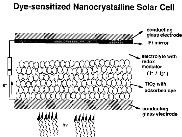
Fig. 5. A cartoon of the make-up of the present generation of dye-sensitized photoelectrochemical cells.
