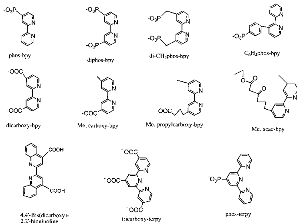
Fig. 4. Various types of polypyridine ligands with carboxyl or phosphonate groups that are being used in solar cell studies.
