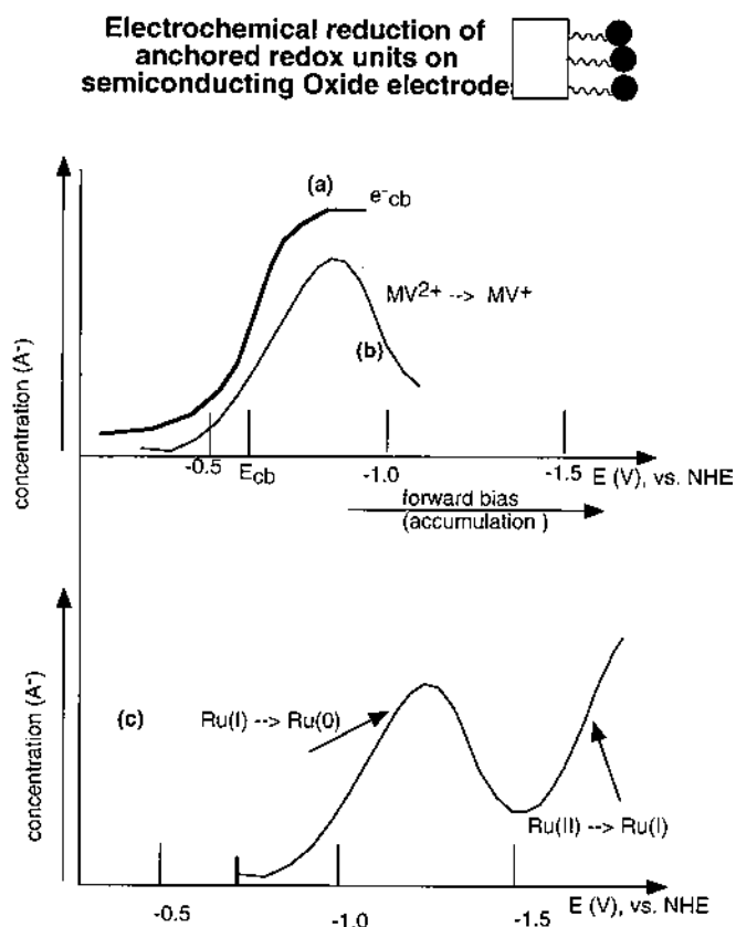
Fig. 11. Schematic presentation of redox processes that occur on anchored redox molecules during potentiostatic control of nanocrystalline oxide electrodes such as TiO_2 . (a) Accumulation of electrons in the conduction band of TiO_2 under forward bias conditions. (b) Electrochromical reduction of viologen anchored onto TiO_2 under forward bias. (c) Electrochemical reduction of phosphanato-bpy complex of Ru(II) anchored on TiO_2 .
