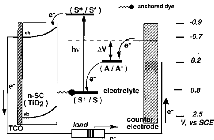
Fig. 3. A schematic presentation of key reactions taking place in a dye-sensitized solar cell.
