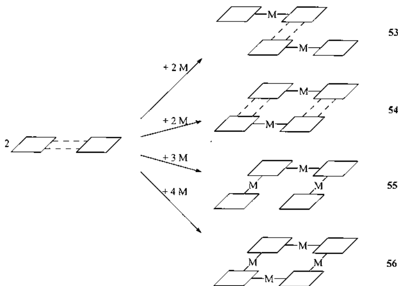
Scheme 6.
