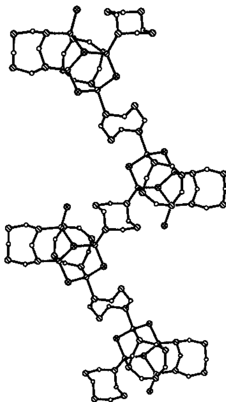
Fig. 34. The polymer chain structure of {}^1_{\infty}[\text{Cu}_4\text{Cl}_4\{\text{cyclo}-(\text{C}_2\text{H}_5\text{AsO})_4\}_3] [42] in which ethyl groups have been omitted for the sake of clarity.
