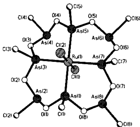
Fig. 18. Molecular structure of [RuCl 2 {cyclo-(CH 3 AsO) 8 }] [46].
