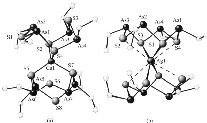
Fig. 42. Molecular structures of the cations of (a) [\text{Cu}\{\text{cyclo}-(\text{C}_2\text{H}_5\text{AsS})_4\}_2]\text{CF}_3\text{SO}_3 [69] and (b) [\text{Ag}\{\text{cyclo}-(\text{C}_2\text{H}_5\text{AsS})_4\}_2]\text{CF}_3\text{SO}_3 [12].
