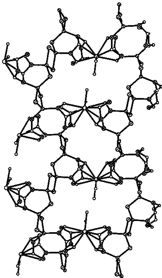
Fig. 31. Packing diagram for the anionic chains that are linked through [Cs{ cyclo -(CH 3 AsO) 4 } 2 ] + sandwiches into a porous sheet in [Cs(H 2 O) 2 ][Cu 3 I 4 { cyclo -(CH 3 AsO) 4 } 2 ] [43]. Methyl groups have been omitted for clarity.
