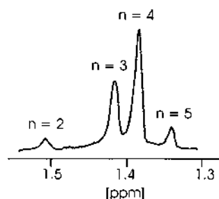
Fig. 1. ^1\text{H} -NMR spectrum (60 MHz) of a \text{CCl}_4 solution of (\text{CH}_3\text{AsO})_n with the assignment of individual resonances to cyclic oligomers of nuclearity n [7].
