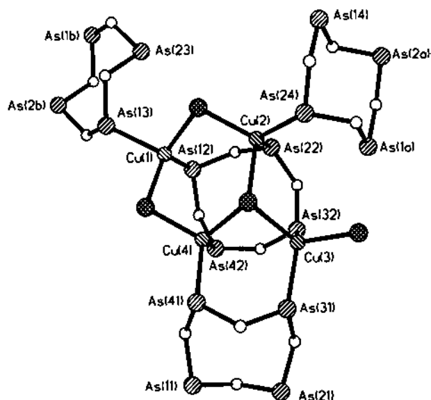
Fig. 13. The asymmetric unit of {}^1_{\infty}[\text{Cu}_4\text{Cl}_4\{\text{cyclo}-(\text{C}_2\text{H}_5\text{AsO})_4\}_3] with the three cyclo-tetramers (\text{C}_2\text{H}_5\text{AsO})_4 of differing bridging mode: bc12 [As31, As41], tc13 [As24, As2a and As13, As1b] and cr4 [As12–As42]. Linkage to an infinite chain is through As(1b) and As(2a) [42].
