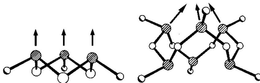
Fig. 7. Directions of lone pairs available for As–M coordination by methylcycloarsoxane: (a) as a cyclootrimer in its preferred chair conformation, (b) as a cyclohexamer with a flattened cuboctahedral conformation.
