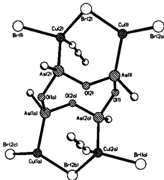
Fig. 12. tc4 bridging mode of the (\text{CH}_3\text{AsO})_4 cyclotetramers in \infty[\{\text{CuBr}(\text{CuBr}-\text{CH}_3\text{CN})_2\}\{\text{cyclo}-(\text{CH}_3\text{AsO})_4\}] [41].
