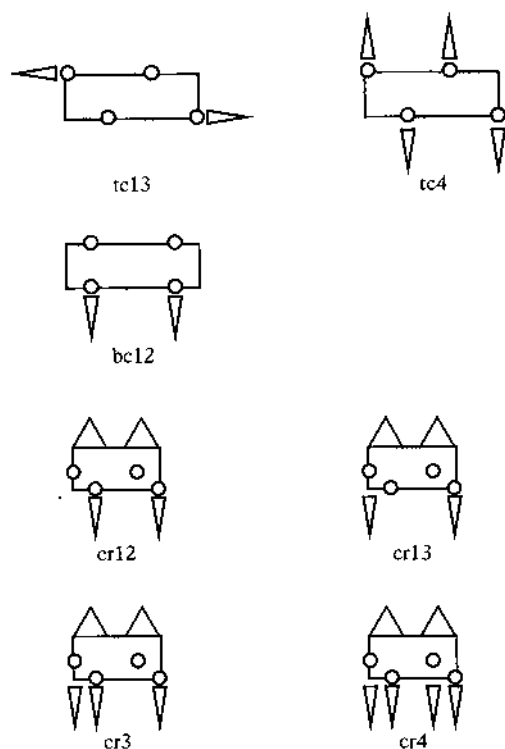
Fig. 10. Schematic representations of (\text{RAsO})_4 bridging modes: \text{tc13} = \mu:1\kappa\text{As}^1:2\kappa\text{As}^3 twist-chair; \text{tc4} = \mu_4:1\kappa\text{As}^1:2\kappa\text{As}^2:3\kappa\text{As}^3:4\kappa\text{As}^4 twist-chair; \text{bc12} = \mu:1\kappa\text{As}^1:2\kappa\text{As}^2 boat-chair; \text{cr12} = \mu-1\kappa\text{As}^1:2\kappa\text{As}^2 crown; \text{cr13} = \mu-1\kappa\text{As}^1:2\kappa\text{As}^3 crown; \text{cr3} = \mu_3-1\kappa\text{As}^1:2\kappa\text{As}^2:3\kappa\text{As}^3 crown; \text{cr4} = \mu_4-1\kappa\text{As}^1:2\kappa\text{As}^2:3\kappa\text{As}^3:4\kappa\text{As}^4 crown.
