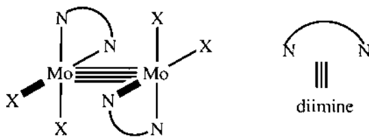
Scheme 5. Proposed structure for \alpha - \text{Mo}_2\text{X}_4(\text{diimine})_2 .
