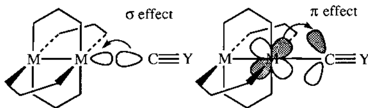
Scheme 4. Activation of axial substrate.
