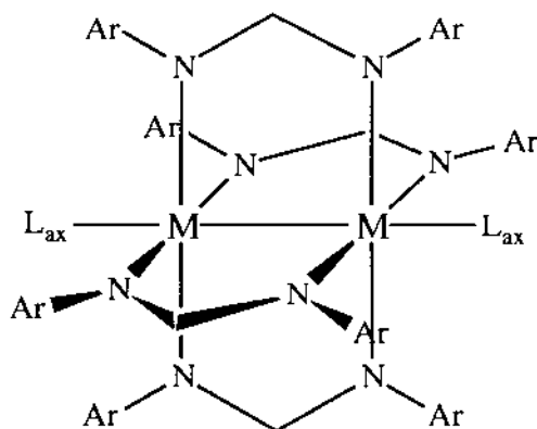
Scheme 2. Paddlewheel motif for M_2(\text{form})_4(L_{\text{ax}})_2 .
