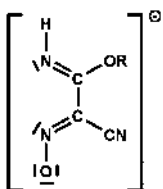
6: (\text{mcoe})^-
