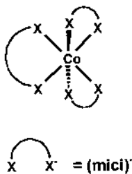
14: [\text{Co}(\text{mici})_3]
