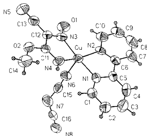
Fig. 6. Molecular structure of [\text{Cu}(\text{mcoe})(\text{bpy})\{\text{N}(\text{CN})_2\}] (courtesy of M. Dunaj-Jurčo). Ellipsoids correspond to 50% probability levels; hydrogen atom radii are arbitrary.
