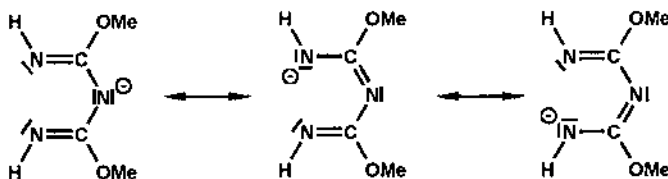
4: (\text{mici})^-
