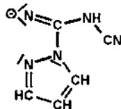
7: \{\text{pz}\cdot\text{N}(\text{CN})_2\}^-
