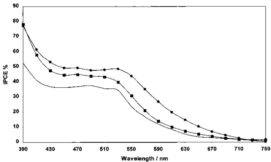
Fig. 9. Photocurrent action spectra obtained for nanocrystalline TiO 2 films coated with cis -[(dcbH 2 ) 2 Ru(isq) 2 ](ClO 4 ) 2 (—), [(dcbH 2 ) 2 Ru(ppy) 2 ](ClO 4 ) 2 (- -) or [(dcbH 2 ) 2 Ru(ppy)(H 2 O)](ClO 4 ) 2 (-●-) as sensitizers in a thin-layer sandwich-type solar cell.
