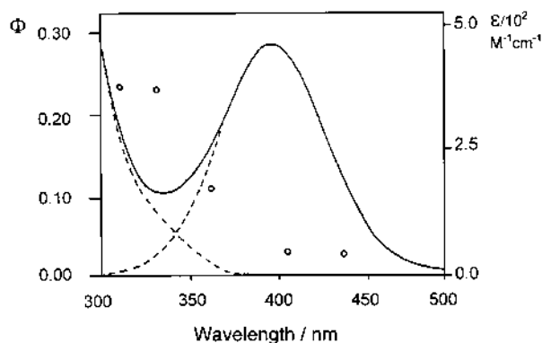
Fig. 1. Quantum yields for the ring closure process in the [Fe(CN)_5(tn)]^{3-} complex for 313, 334, 365, 404 or 434 nm irradiation. The dashed line represents the Gaussian deconvolution of the electronic spectrum.
