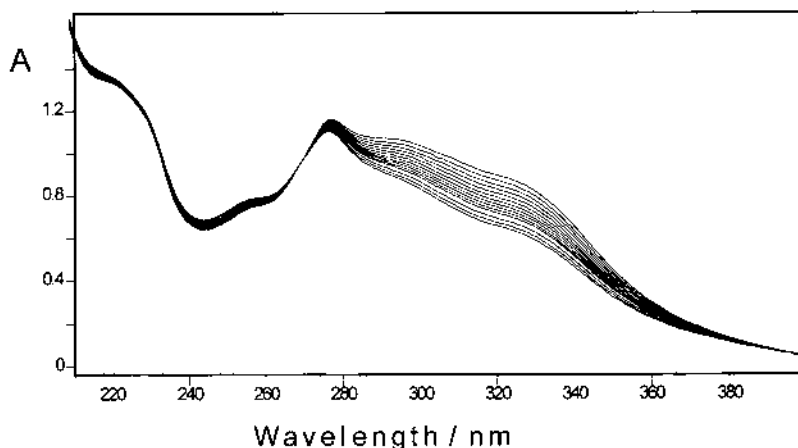
Fig. 4. Spectral changes during the 313 photolysis of 1.67 \times 10^{-4} M [\text{Re}(\text{CO})_3(\text{phen})(t\text{-bpe})]\text{PF}_6 in \text{CH}_3\text{OH} . T = 298 K, \Delta t_{\text{irr}} = 5 s.
