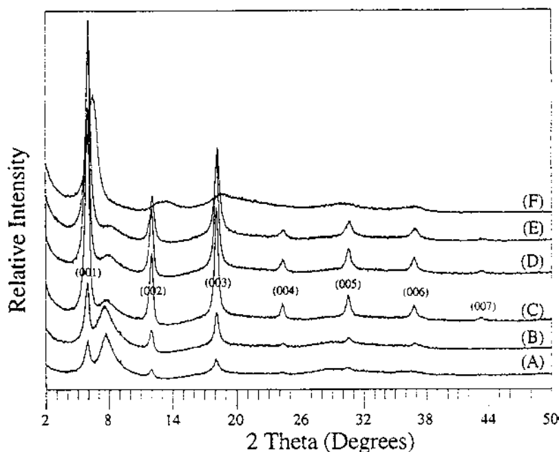
Fig. 18. XRD patterns ( \text{Cu-K}_\alpha ) of oriented film samples of \text{Mg,Al-LDH} metatungstate reaction products obtained from (A) meixnerite, (B) LDH glycerolate, and (C) LDH triethyleneglycolate precursors. All diffraction patterns were recorded at r.t. For the LDH-POM intercalated derived from the triethyleneglycolate precursors, the XRDs were taken at r.t. after 1 h preheating under nitrogen at (D) 100, (E) 200, and (F) 250°C. Reprinted from S.K. Yun, V.R.L. Constantino, T.J. Pinnavaia, New polyol route to keggion ion-pillared layered double hydroxides, Microporous Mater. 4 (1995) 21–29, © 1995, with permission from Elsevier Science.
