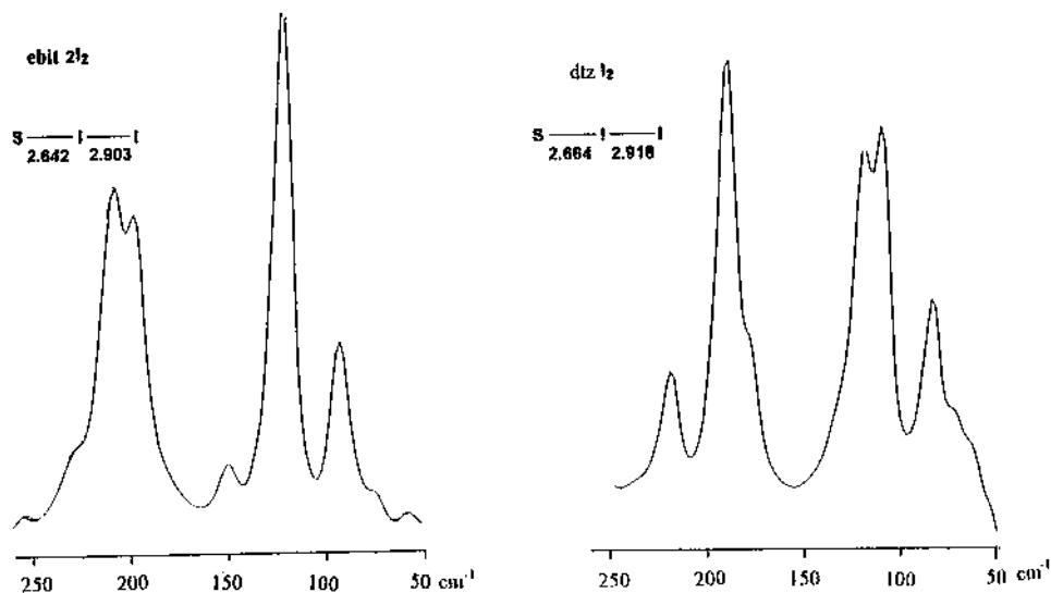
Fig. 5. Examples of FT-Raman spectra of type 2 adducts \text{ebit} \cdot 2\text{I}_2 [ \text{ebit} = 1,1'-ethylenebis(3-methyl-4-imidazoline-2-thione)] and \text{dtz} \cdot \text{I}_2 ( \text{dtz} = dithizone), where two groups of bands occur near 200 and 120 \text{cm}^{-1} and are assigned to the antisymmetrical and symmetrical stretching of the S–I–I moiety, respectively.
