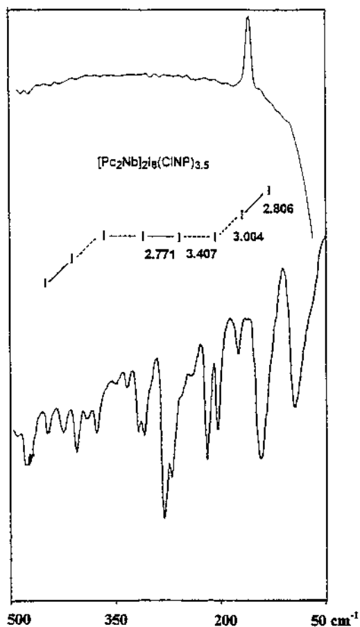
Fig. 9. Comparison of the FT-Raman (upper, \nu_{I-I} = 167 \text{ cm}^{-1} assigned to the less elongated I_2 ) and Far-IR spectra (lower, \nu_{I-I} = 144 \text{ cm}^{-1} assigned to the more elongated I_2 ) of [Pc_2Nb]_2I_8(CINP)_{3.5} , (Pc = phtalocyanine, CINP = \alpha -chloronaphtalene).
