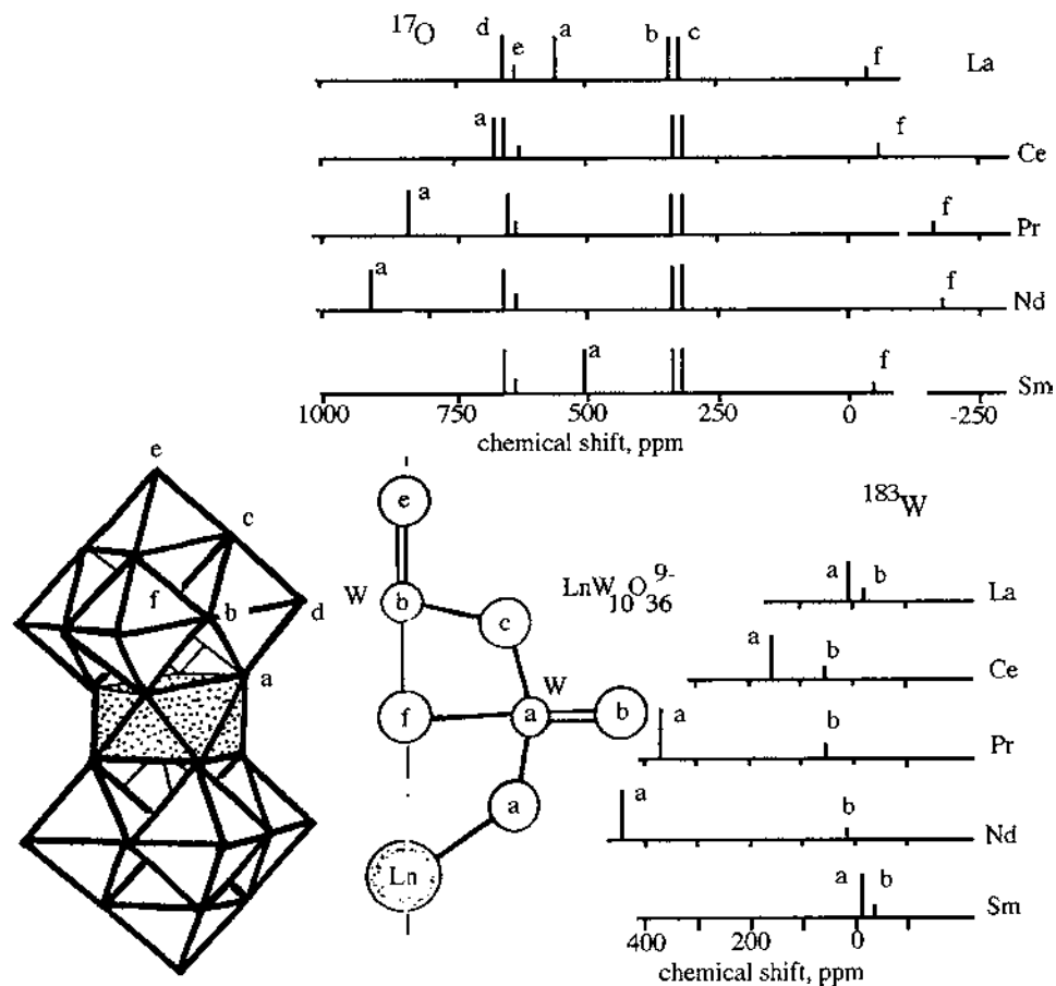
Fig. 3. The structure and fragment of \text{XW}_{10}\text{O}_{36}^{n-} and ^{17}\text{O} - and ^{183}\text{W} -NMR chemical shift diagram.
