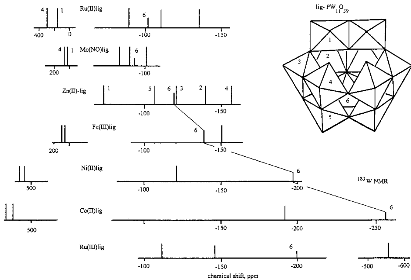
Fig. 6. The structure of \text{PW}_{11}\text{MO}_{39}^{9-} and ^{183}\text{W} -NMR chemical shift diagram.
