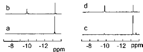
Fig. 2. Proton NMR spectra of the probe with dGMP and \text{Cp}_2\text{TiCl}_2 in \text{D}_2\text{O} . Left, drug:dGMP:probe = 1:1:1, dGMP, 0.001 \text{ mol l}^{-1} ( \text{pD} = 6.44 ) (a) after 20 min; (b) after 24 h; Right, drug:dGMP:probe = 0.5:1:1, dGMP, 0.001 \text{ mol l}^{-1} ( \text{pD} = 6.94 ); (c) after 20 min; (d) after 24 h.
