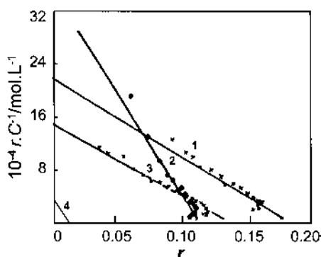
Fig. 7. Scatchard plots. 1–4, R_t : 0, 0.25, 0.5, 1.0, respectively.
