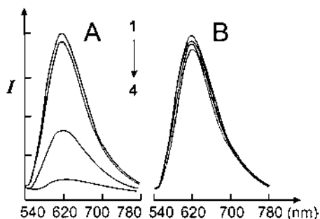
Fig. 6. Fluorescence spectra of calf thymus DNA-EB in the presence of varying concentration of \text{Cp}_2\text{TiCl}_2 or \text{Cp}_2\text{ZrCl}_2 . (A) \text{Cp}_2\text{TiCl}_2 ; (B) \text{Cp}_2\text{ZrCl}_2 ; 1–4 R_t : 0, 0.5, 1, 2, respectively.
