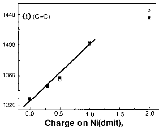
Fig. 3. Frequency shift of the C=C stretching mode as a function of the formal charge on the [M(dmit)_2]^{n-} anion in M(dmit)_2 based compounds (■: M = Ni; ○: M = Pd).
