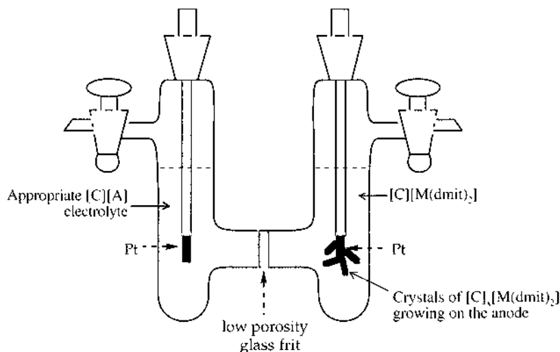
Fig. 1. Electrolysis cell.
