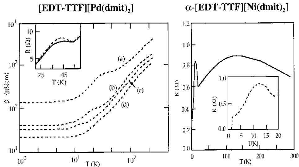
Fig. 5. Anomalous resistivity maximum at ca. 40 K for (EDT-TTF)[Pd(dmit) 2 ] (for an injected current I of 150 \mu A at (a) ambient pressure, 2 kbar; (b) 5 kbar; (c) 10 kbar; (d) the insert shows the non-Ohmic behavior observed at ambient pressure for I=150 (···) and 1.5 (—) \mu A), and at ca. 14 K for \alpha -(EDT-TTF)[Ni(dmit) 2 ] (the inset shows the data below 20 K). Redrawn after [37] and [38].
