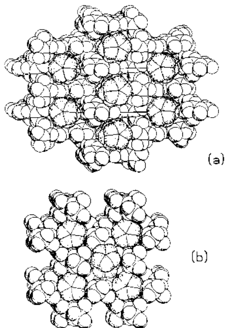
Fig. 10. The hexagonal and tetragonal superanions molded around cobalticinium cations in crystalline [(\eta^5\text{-C}_5\text{H}_5)_2\text{Co}]^+[(\text{D,L-HTA})(\text{D,L-H}_2\text{TA})]^- (a) and [(\eta^5\text{-C}_5\text{H}_5)_2\text{Co}]^+[\text{L-HTA}]^- (b) ( \text{D,L-H}_2\text{TA} = \text{D,L-tartaric acid} ).
