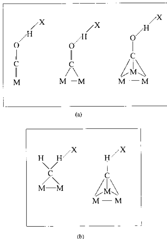
Fig. 6. Scheme of the hydrogen bonding interactions of the terminal \text{CO}\cdots\text{H} , \mu_2\text{-CO}\cdots\text{H} , and \mu_3\text{-CO}\cdots\text{H} type (a) and of the \mu_2\text{-CH}_2\cdots\text{O} and \mu_3\text{-CH}\cdots\text{O} type (b).
