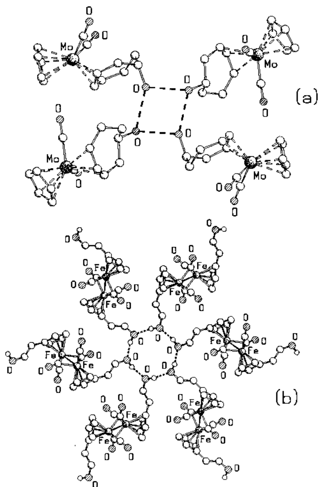
Fig. 4. Tetrameric (-\text{O}-\text{H})_4 (a) and hexameric (-\text{O}-\text{H})_6 (b) hydrogen bond rings are observed also for metal coordinated ligands.
