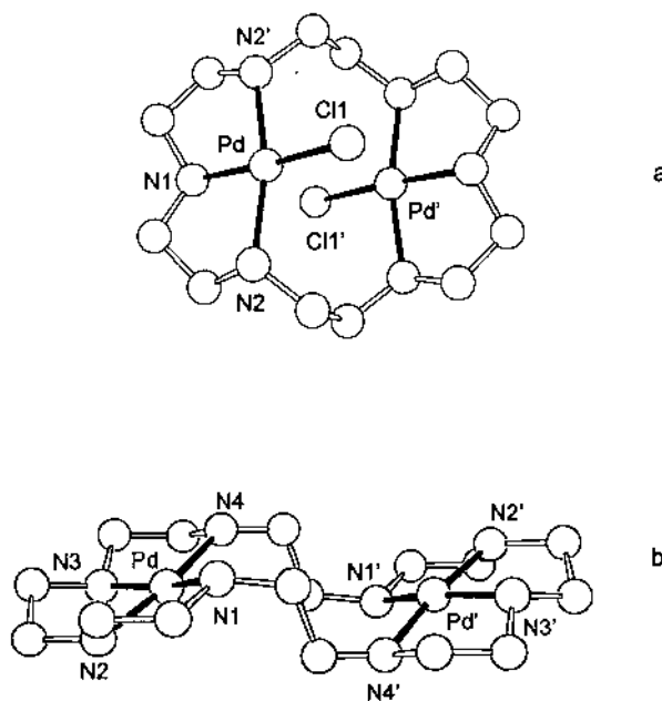
Fig. 9. Crystal structures of (a) [\text{Pd}_2([18]\text{aneN}_6)\text{Cl}_2]^{2+} and (b) [\text{Pd}_2([24]\text{aneN}_8)]^{4+} . Selected bond distances (Å) and angles (°) for (a): Pd–N1 1.99, Pd–N2 2.049, Pd–Cl1 2.301, Pd–Pd' 3.04; N1–Pd–N2 83.9, Cl1–Pd–N2 95.6, N2–Pd–N2' 166.5, N1–Pd–Cl1 171.4 [11]. Selected bond distances (Å) and angles (°) for (b): Pd–N1 2.10, Pd–N2 1.98, Pd–N3 1.99, Pd–N4 2.04, Pd–Pd' 5.447; N3–Pd–N4 86.7, N2–Pd–N4 171.4, N2–Pd–N3 85.4, N1–Pd–N4 164.4, N1–Pd–N3 164.4, N1–Pd–N2 84.0, N1–Pd–N3 179.4, N2–Pd–N4 167.2 [12].
