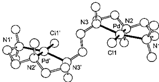
Fig. 6. Crystal structure of [\text{Pd}_2(\text{Me}_8(2,2,2,2,2\text{-hexa}))\text{Cl}_2]^{2+} . Selected bond distances (Å) and angles (°): Pd–Cl1 2.306, Pd–N1 2.063, Pd–N2 2.049, Pd–N3 2.074; N2–Pd–N3 86.6, N1–Pd–N2 86.0, Cl1–Pd–N3 93.5, Cl1–Pd–N1 94.4, N2–Pd–Cl1 177.4, N1–Pd–N3 165.6 [7].
