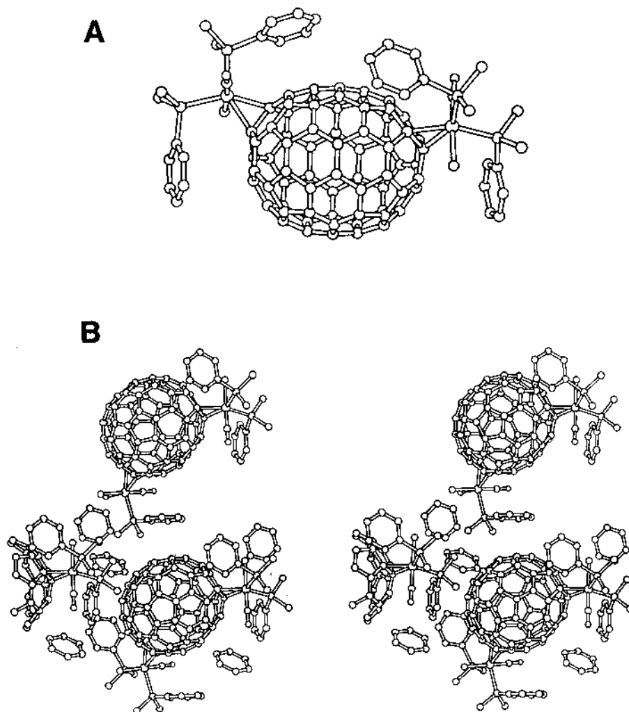
Fig. 1. (A) A view of the adduct (C_{70})\{Ir(CO)Cl(PhPMe_2)_2\}_2 . (B) A portion of the solid state structure of (C_{70})\{Ir(CO)Cl(PhPMe_2)_2\}_2 \cdot 3C_6H_6 in which the C_{60} /phenyl interactions are emphasized. Taken with permission from the Ph.D. Thesis of J.W. Lee, University of California, Davis, CA, USA, 1994. See also A.L. Balch, J.W. Lee, M.M. Olmstead, Angew. Chem. Int. Ed. Engl. 31 (1992) 1356.
