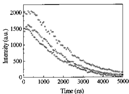
Fig. 11. The time-resolved emission decays of [\text{Ru}(\text{bpy})_2(\text{MCP})]^{2+} ( 2\ \mu\text{M} ) in the DNA ( 200\ \mu\text{M} nucleotide) as a function of added quencher (0, 6 and 7\ \mu\text{M} [\text{Ru}(\text{bpy})_2(\text{MNP})]^{2+} from top to bottom).
