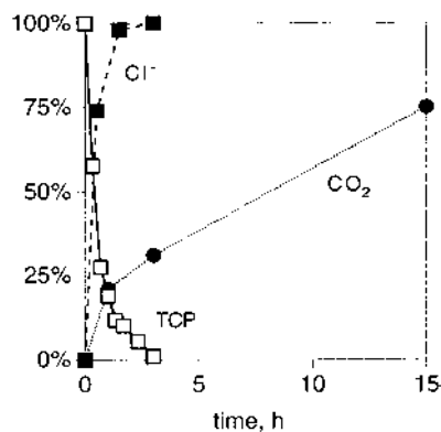
Fig. 6. Time course for the oxidation of 2,4,6-trichlorophenol (TCP), 10 mM, by \text{H}_2\text{O}_2 , 300 mM, in water pH 7.5 (phosphate buffer); RuPcS catalyst (1 mM); 20°C.
