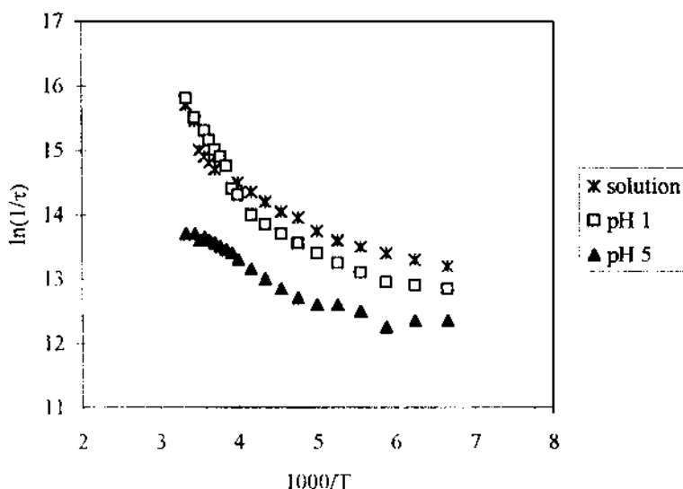
Fig. 3. Temperature dependence for the luminescent lifetime of 5 in \times , 4:1 ethanol/methanol; \square , pH 1 sol-gel; \blacktriangle , pH 5 sol-gel in the temperature range 150–300 K.
