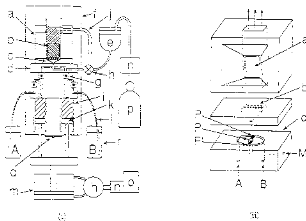
Fig. 2. (i) Block diagram of stopped-flow assembly: (a) observation cell; (b) window; (c) nozzle; (d) mixing chamber; (e) medium solution vessel; (f) thermostated block; (g) ruby ball; (h) electromagnetic two-way valve; (i) piston cylinder; (j) drain; (k) piston head; (l) Teflon tube; (m) gas cylinder, (n) pressure regulator; (o) air compressor; (p) nitrogen gas cylinder; (q) microswitch; (r) reservoir. A and B are a medium solution containing the mercury–porphyrin complex with an acetate buffer of ca. pH 5.8 and a solution containing divalent metal ions, respectively. (ii) Block diagram of observation cell and mixing chamber: (a) window made of boron nitride; (b) nozzle; (c) mixing chamber. A and B are the two solutions given in (i). P and P' are three point outlets of solutions in the mixing chamber.
