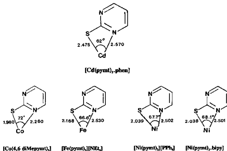
Scheme 10.
