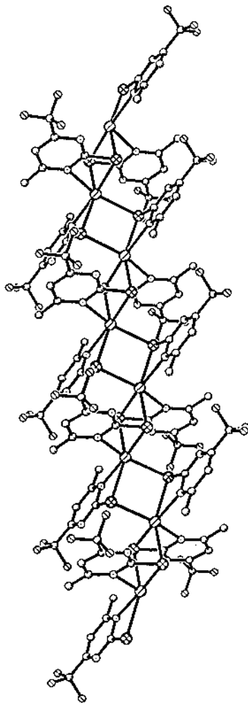
Fig. 34. The structure of the complex [\text{Cd}(4,6\text{-MeCF}_3\text{pymS})_2] (adapted from Ref. [55]).
