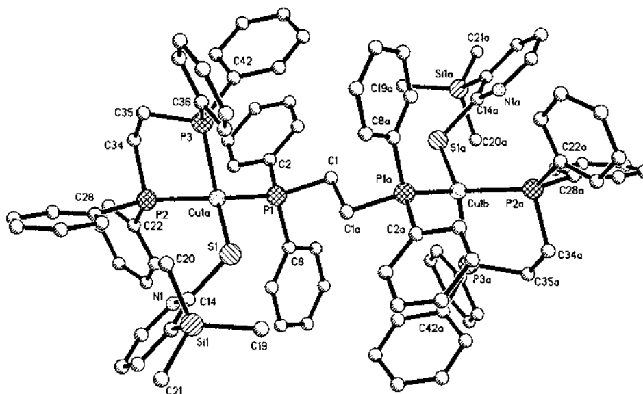
Fig. 24. Molecular structure of [\text{Cu}_2(3\text{-Me}_3\text{SipyS})_2(\text{dppe})_3] (adapted from Ref. [41]).
