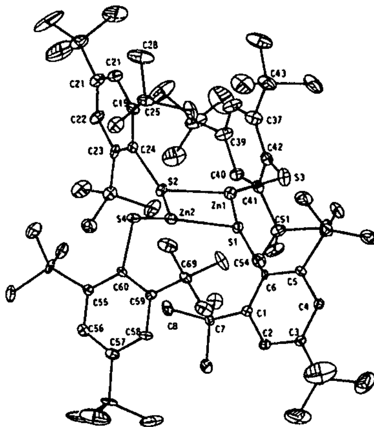
Fig. 3. Molecular structure of [\text{Zn}(\text{S-Bu}_3\text{C}_6\text{H}_2-2,4,6)_2] (adapted from Ref. [13]).
