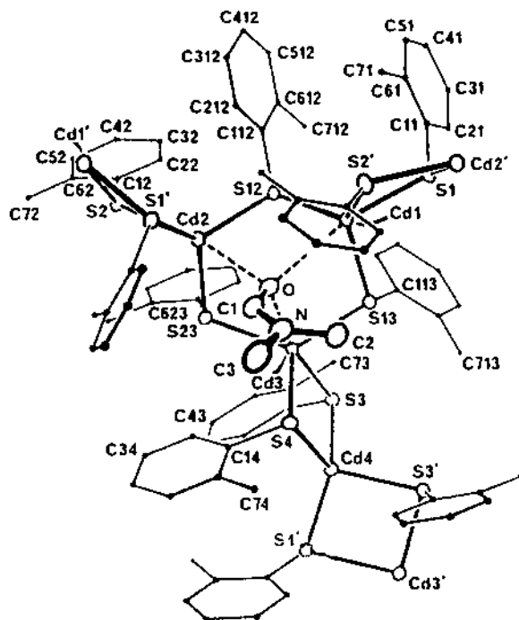
Fig. 2. Molecular structure of [Cd(SPh-2-Me) 2 ] (adapted from Ref. [12]).
