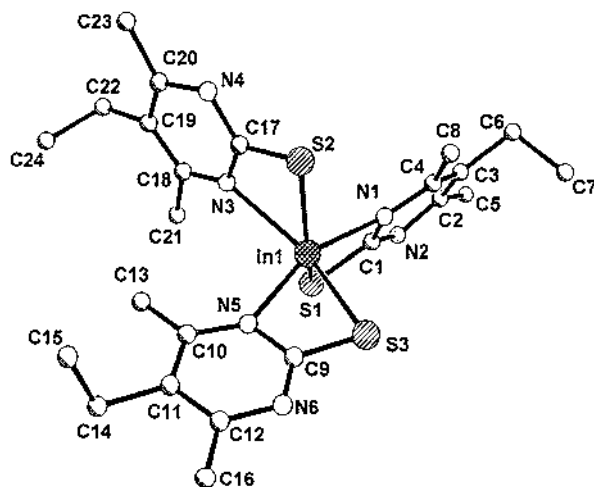
Fig. 48. Molecular structure of [\text{In}(\text{5-Et-4,6-Me}_2\text{pmyS})_3] (adapted from Ref. [98]).
