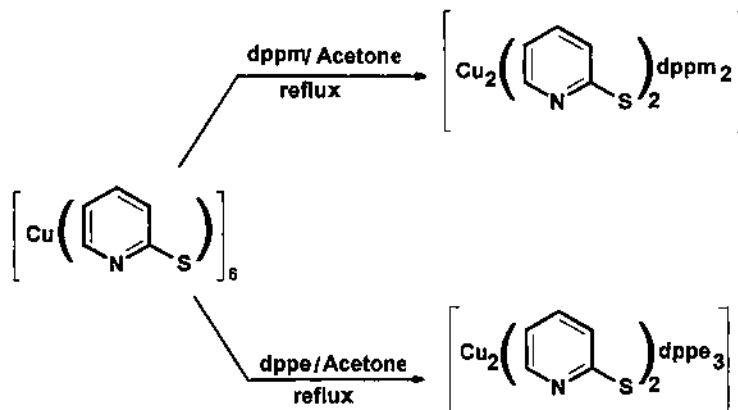
Scheme 7.
