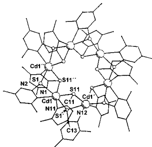
Fig. 30. Perspective view of the structure of [\{\text{Cd}(\text{4,6-Me}_2\text{pymS})_2\}_6] (adapted from Ref. [53]).
