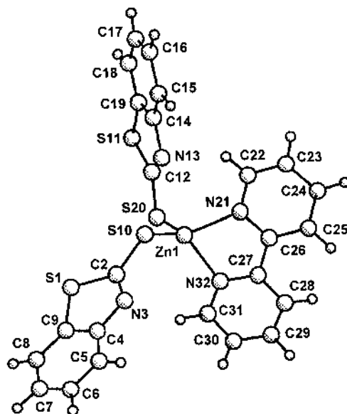
Fig. 38. Molecular structure of [\text{Zn}(\text{bzS})_2(\text{bipy})] (adapted from Ref. [58]).
