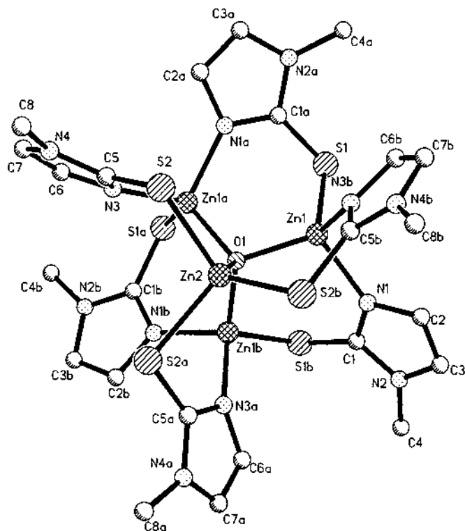
Fig. 29. Perspective view of the [\text{Zn}_4\text{O}(\text{MeImS})_6] molecule (adapted from Ref. [51]).
