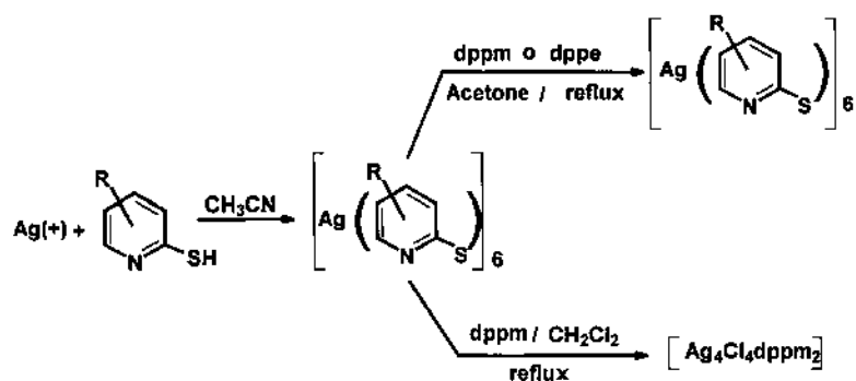
Scheme 8.
