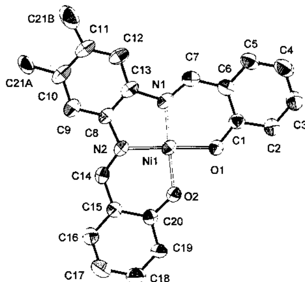
Fig. 26. Molecular structure of \text{Ni}(\text{sal-3,4-toluen}) \cdot 1.5\text{CHCl}_3 . Adapted from Ref. [13].
