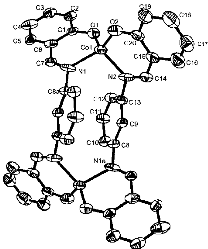
Fig. 27. ORTEP view of the binuclear complex [\text{Co}_2(\text{sal-}m\text{-phen})_2] . Adapted from Ref [101].
