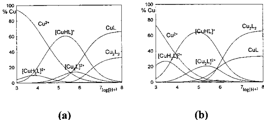
Fig. 18. Species distribution diagram as a function of pH for the system H_2sal -2,6-toluen-Cu(II) at ligand:metal ratio 1:1 (a) C_M = 0.5 mM; (b) C_M = 4.0 mM.
