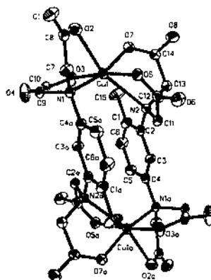
Fig. 12. ORTEP view of the anionic complex [\text{Cu}_2(2,4\text{-TDTA})_2]^{4-} . Adapted from Ref. [64].
