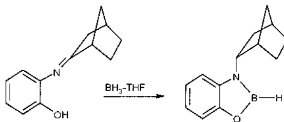
Fig. 68. Preparation of boroxazolines by reducing phenolamines with borane.
