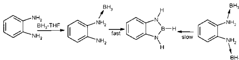
Fig. 74. Reaction products of phenylenediamine and \text{BH}_3 -THF.
