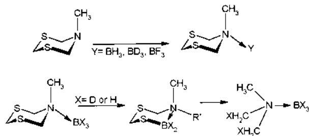
Fig. 77. Dithiazine N-boron adducts and ring reactions.
