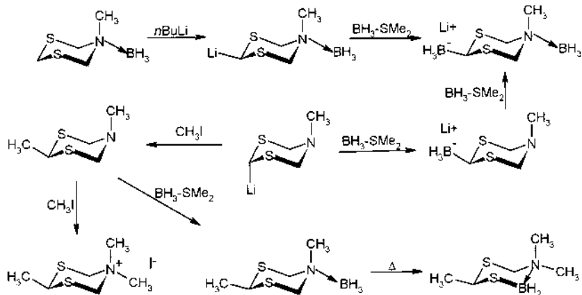
Fig. 78. Reactions at C-2 and at nitrogen atom of dithiazines with \text{BH}_3 -DMS.
