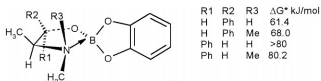
Fig. 36. Spiranic compounds derived from catecholborane and ephedrine, the free activation enthalpy of the B–N bonds obtained by VT-NMR measurements are shown.
