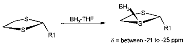
Fig. 46. ^{11}\text{B} -NMR shifts (ppm) and stereoisomers of \text{S}-\text{BH}_3 adducts of dithiolanes.
