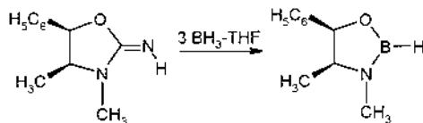
Fig. 54. Boroxazoline prepared from oxazolidine-2-imino ephedrine.
