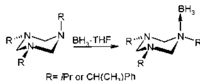
Fig. 82. Stereochemistry of borane addition to triazines.
