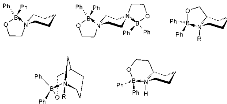
Fig. 89. Diphenylborinic esters derived from methanol or ethanol piperidines or piperazines.
