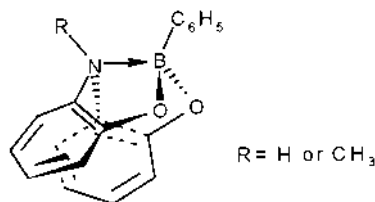
Fig. 28. Structure of 2,2'-diphenolamine phenylboronic esters.
