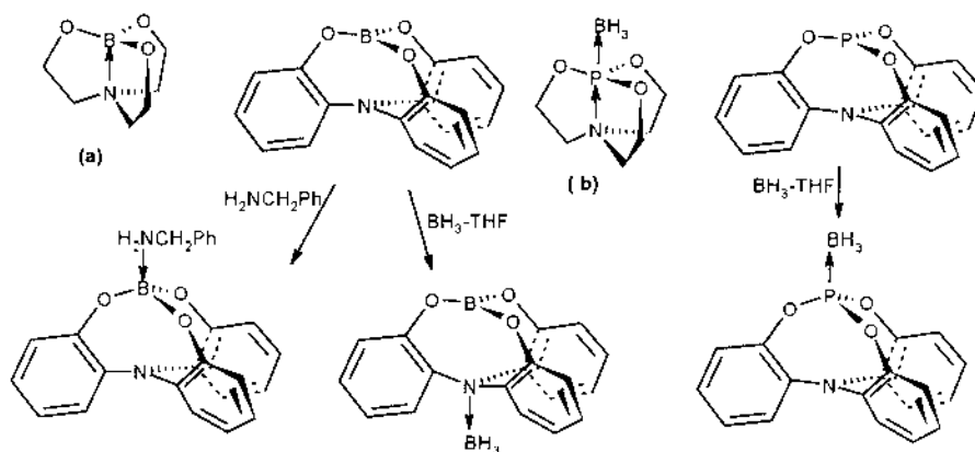
Fig. 41. Bora- and phosphapseudoatranes derived from triphenolamine. The structures are compared with those of (a) bora- [60] and (b) phosphatranes [61].
