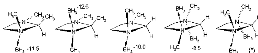
Fig. 45. ^{11}\text{B} -NMR shifts (ppm) and stereoisomers of \text{N}-\text{BH}_3 adducts of diazolidines, ^{11}\text{B} signal was not observed.
