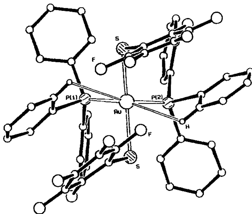
Fig. 1. X-ray diffraction structure of [Ru(SX) 2 (PPh 3 ) 2 ]. Reprinted from Ref. [26] with permission from Elsevier Science.
