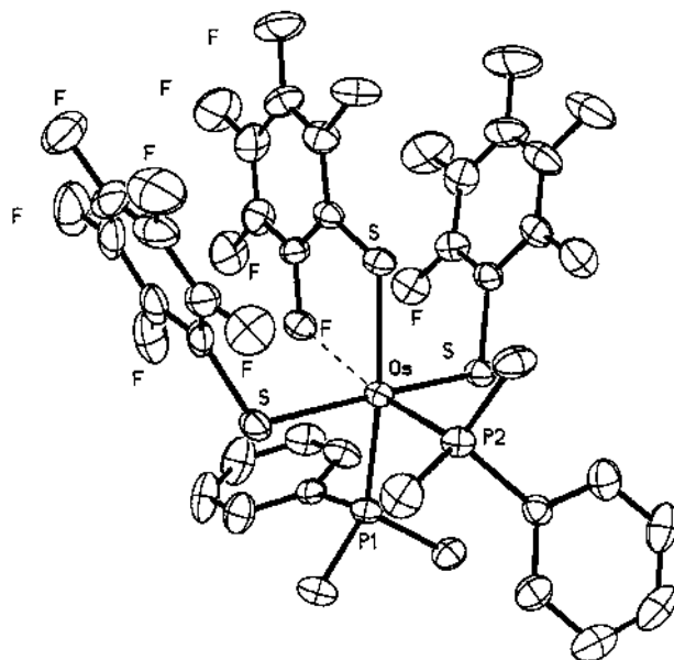
Fig. 5. X-ray diffraction structure of [\text{Os}(\text{SX})_3(\text{PMe}_2\text{Ph}_2)_2] . Reprinted from Ref. [36] with permission from Elsevier Science.
