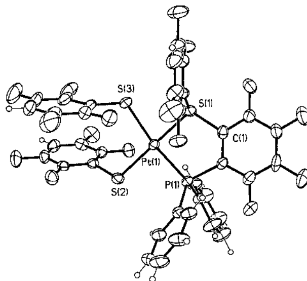
Fig. 15. X-ray diffraction structure of [\text{Pt}(\text{SX})_2(o\text{-(Ph}_2\text{P)(XS)C}_6\text{F}_4)] [79].
