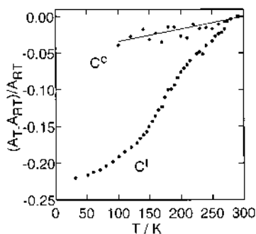
Fig. 2. Temperature dependence of the relative absorbance (A_T - A_{\text{RT}})/A_{\text{RT}} at 342 nm for the \text{C}^{\text{c}} and \text{C}^{\text{t}} forms of \text{Fe}(\text{stpy})_4(\text{NCBPh}_3)_2 embedded in cellulose acetate films.
