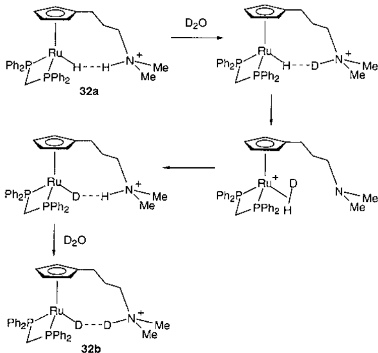
Scheme 1.
