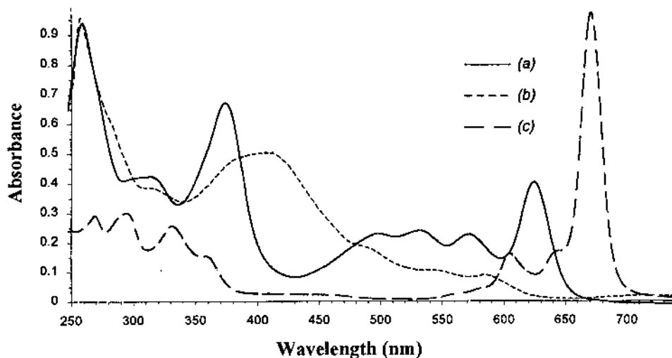
Fig. 1. UV-vis spectra of (a) 8a in chloroform, c = 2.1 \times 10^{-5} \text{ mol l}^{-1} , (b) 8a in trifluoroacetic acid, c = 2 \times 10^{-5} \text{ mol l}^{-1} and (c) nickel tetra- tert -butylphthalocyanine in chloroform, c = 3.4 \times 10^{-6} \text{ mol l}^{-1} .
