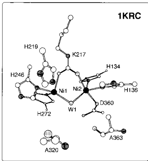
Fig. 6. Model of the active site of KAU His ^{\alpha 320} Ala mutant, showing the position of selected relevant residues. Atoms and bonds as in Fig. 1. All residues are sized according to their different depths. The PDB code is indicated.
