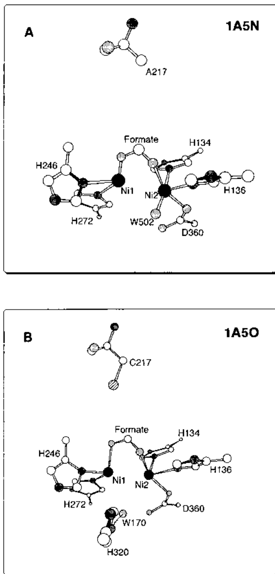
Fig. 10. Model of the active site of KAU Lys \alpha 217 Ala (A) and Lys \alpha 217 Cys (B) mutants chemically rescued with formate, showing the position of selected relevant residues. Atoms and bonds as in Fig. 1. All residues are sized according to their different depths. The PDB code is indicated.
