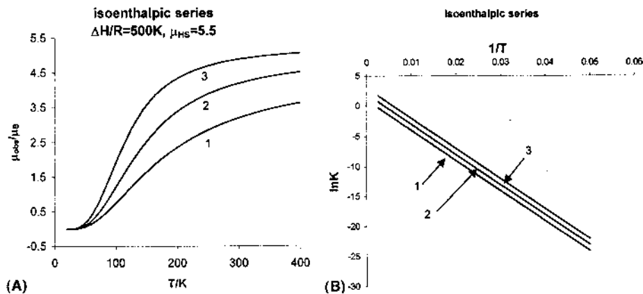
Fig. 14. Isoenthalpic series of spin-crossover equilibria. No intersection point of van't Hoff plots ( \Delta H/R = 500 K, \mu_{\text{HS}} = 5.5 ; 1: \Delta S/R = 1 ; 2: \Delta S/R = 2 , and 3: \Delta S/R = 3 ): (A) \mu vs. T curves; (B) van't Hoff plots.
