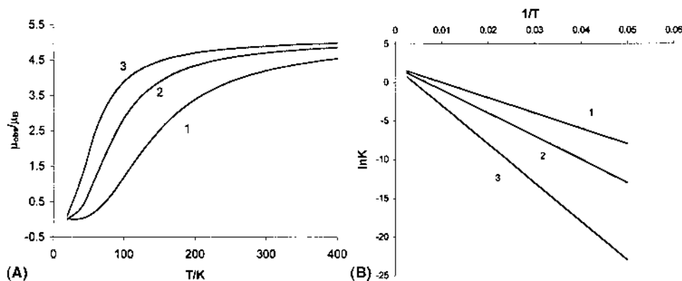
Fig. 15. Isoentropic series of spin-crossover equilibria ( \Delta S/R = 2 , \mu_{\text{HS}} = 5.5 ; 1: \Delta H/R = 500 K; 2: \Delta H/R = 300 K; and 3: \Delta H/R = 200 K): A, \mu vs. T curves; B, van't Hoff plots.
