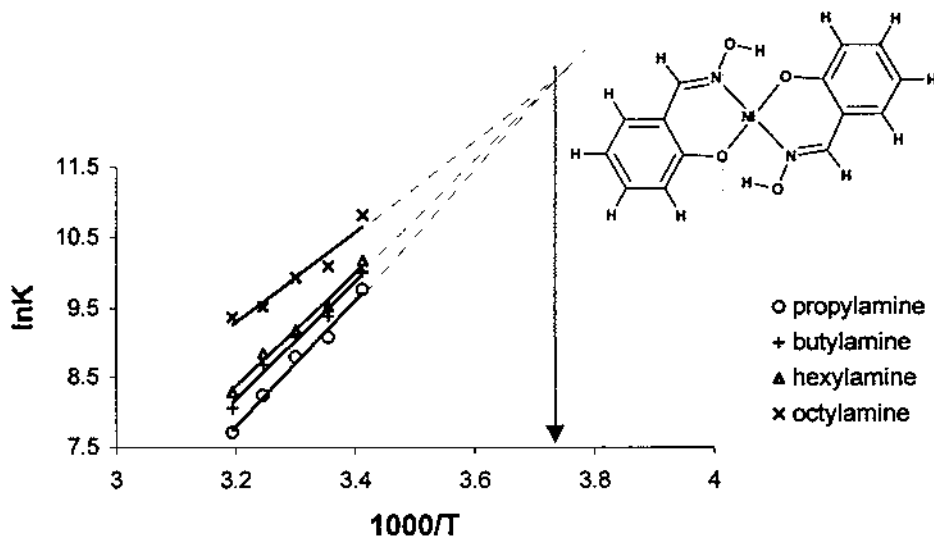
Fig. 23. Isoequilibrium relationship in the series of adducts of bis-(salicylaldoximato)nickel(II) [\text{Ni}(\text{Saldox})_2] with amines.
