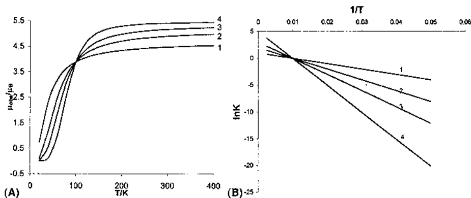
Fig. 12. A series of spin–crossover equilibria exhibiting intersection point (isoequilibrium point) in the range of experimental data (compensation \delta\Delta H/\delta\Delta S = 100 K, \mu_{HS} = 5.5 ; 1: \Delta H/\Delta S = 100/1 ; 2: \Delta H/\Delta S = 200/2 ; 3: \Delta H/\Delta S = 300/3 ; and 4: \Delta H/\Delta S = 500/5 ): A, \mu vs. T curves; B, van't Hoff plots.
