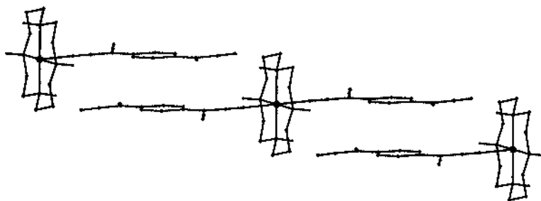
Fig. 4. Linear chains by TCNQ dimerization in [\text{Ni}([14]\text{aneN}_4)(\text{TCNQ})_2] , Ref. [30].
