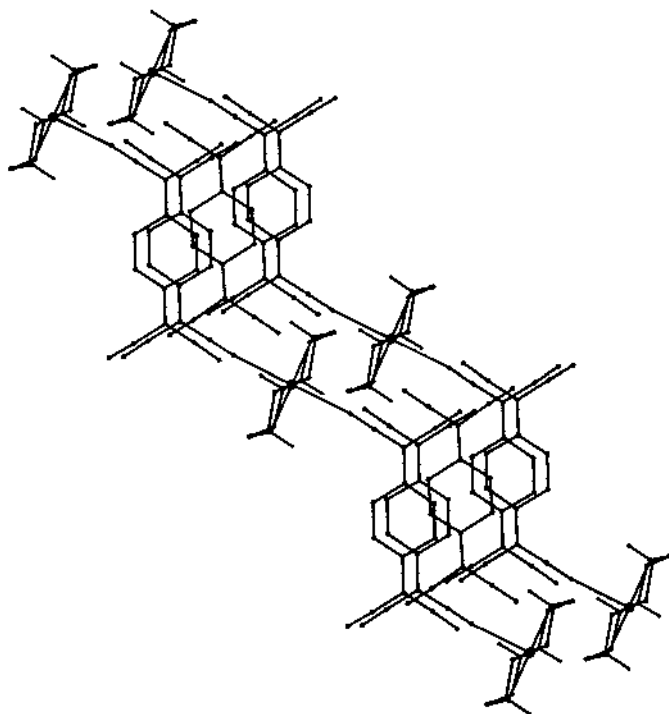
Fig. 10. Overlapping of neutral and anionic TCNQ in [\text{Cu}([14]\text{aneN}_4)(\text{TCNQ})_3] , polymorph 1, Ref. [47].
