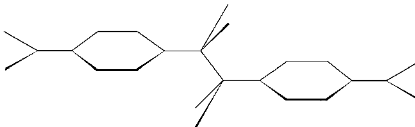
Fig. 7. Formation of \sigma bond in the (\text{TCNQ})_2 dimers.
