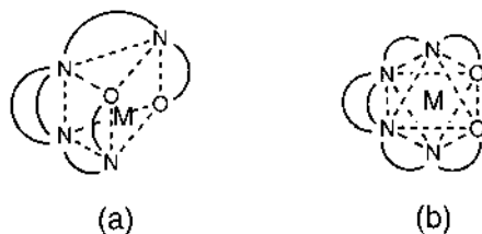
Fig. 1. Extreme configurations, TP(a) and ATP(b) of [M(\text{Sal-prpi})]^+ : (a) M = \text{Fe(III)} ; (b) M = \text{Co(III)} .
