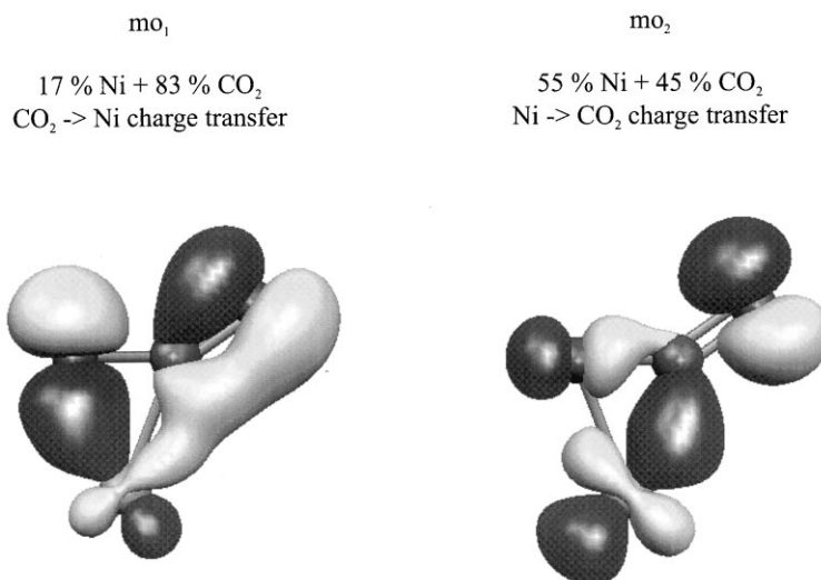
Fig. 4. The bonding orbitals of \eta^2(\text{C,O}) \text{Ni}(\text{CO}_2) .
