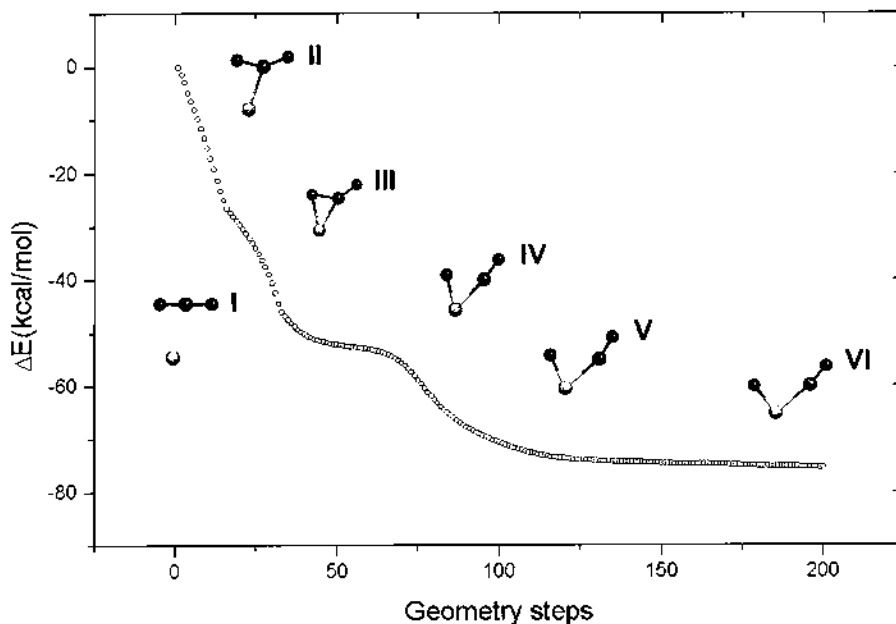
Fig. 7. The variation of the total energy along the \text{Ti}(s^2d^2) + \text{CO}_2(^1\Sigma_g^+) \rightarrow \text{OTiCO}(^3A') reaction path. The energies are given for each even number of geometry steps relative to the initial structure. Structures corresponding to steps numbered 0, 20, 40, 75, 100, and 200 are referred as structures I–VI, respectively.
