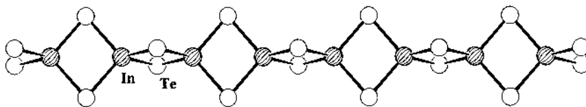
Fig. 4. The {}^1_{\infty}[\text{In}_2\text{Te}_4]^{2-} one-dimensional chain in 4 .
