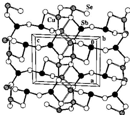
Fig. 14. A view of the {}^2_{\infty}[(\text{Cu}_2\text{Sb}_2\text{Se}_5)^{2-}] two-dimensional layer in 22 .
