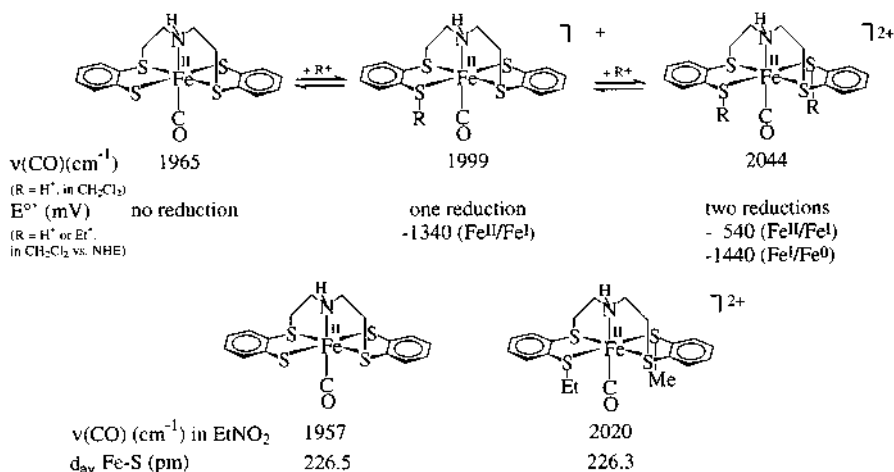
Fig. 2. Electronic, structural, and redox effects in [\text{Fe}(\text{CO})(\text{NH}_4\text{S}_4)] upon reversible protonation ( \text{R} = \text{H}^+ ) or irreversible alkylation ( \text{R} = \text{Me}^+ , \text{Et}^+ ).
