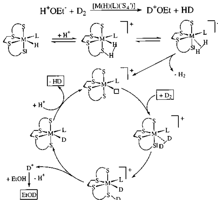
Scheme 1. Mechanism of heterolytic \text{H}_2 activation catalyzed by [\text{M}(\text{H})(\text{L})(\text{S}_4)] complexes ( \text{M} = \text{Rh}, \text{Ru} ; \text{L} = \text{CO}, \text{PCy}_3 ).
