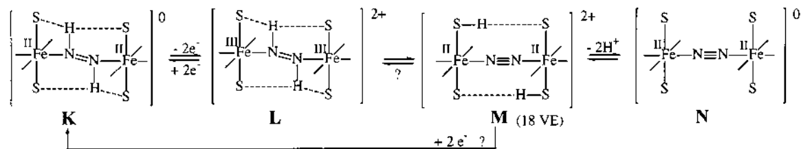
Scheme 4. Redoxisomerism of the [\mu\text{-N}_2\text{H}_2\{\text{Fe}(\text{P}^n\text{Pr}_3)(\text{'S}_4\text{'})\}_2]^{2+} dication.
