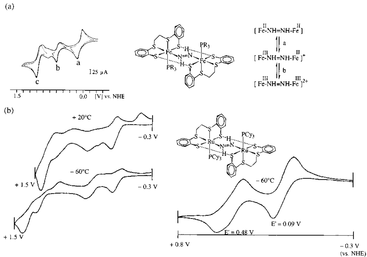
Fig. 5. (a) Cyclic voltammogram of [\mu\text{-N}_2\text{H}_2\{\text{Fe}(\text{PPr}_3)(\text{S}_4')\}_2] at -20^\circ\text{C} ( \text{CH}_2\text{Cl}_2 , v = 20\text{ mV s}^{-1} ) and assignment of (formal) Fe oxidation states. (b) Cyclic voltammograms of [\mu\text{-N}_2\text{H}_2\{\text{Ru}(\text{PCy}_3)(\text{S}_4')\}_2] at +20 and -60^\circ\text{C} ( \text{CH}_2\text{Cl}_2 , v = 50\text{ mV s}^{-1} ) within different scan ranges.
