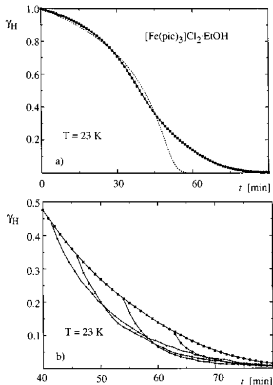
Fig. 8. HS → LS relaxation curves for [Fe(pic) 3 ]Cl 2 ·EtOH at 23 K. (a) Full curve (□) experimental; (---) mean-field prediction. (b) Relaxation curves following a partial population of the HS state with the full curve as reference curve (adapted from Ref. [29]).
