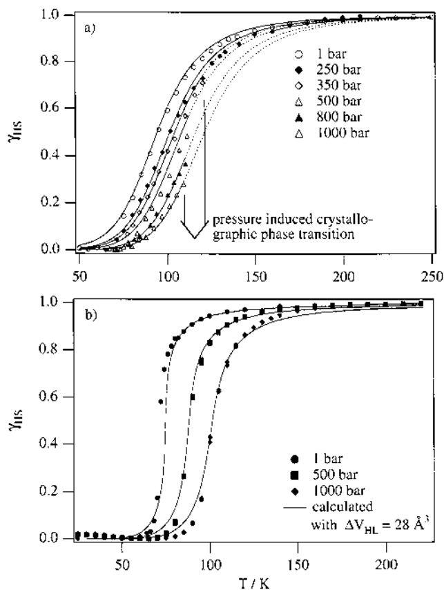
Fig. 5. (a) Thermal transition curves of [Zn_{1-x}Fe_x(ptz)_6](BF_4)_2 ( x = 0.1 ) at ambient pressure and for pressures up to 1 kbar. Samples were cooled to 15 K before applying pressure, transition curves were recorded in the heating mode. Symbols: experimental. Full lines: calculated with \Delta V_{HL} = 26 \text{ \AA}^3 . (b) Thermal transition curves for [Fe(ptz)_6](PF_6)_2 at 1 bar, 500 bar and 1 kbar. Full lines: calculated with \Delta V_{HL} = 28 \text{ \AA}^3 (adapted from Refs. [17,24]).
