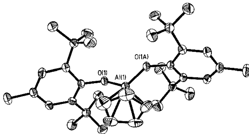
Fig. 8. Molecular structure of \text{CpAl}(\text{BHT})_2 . Reprinted with permission from Ref. [30]. Copyright 1998 The American Chemical Society.
