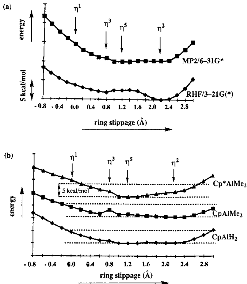
Fig. 10. (a) Energy profile for ring slippage in CpAlH 2 at RHF/3-21G(*) and MP2/6-31G*. (b) Energy profiles for ring slippage of CpAlH 2 , CpAlMe 2 , and Cp*AlMe 2 at MP2/6-31G* (estimated from RHF/3-21G(*) calculations). The ring slippage coordinate is arbitrarily set at 0.0 Å for an η 1 geometry. Reprinted with permission from Ref. [13]. Copyright 1997 The American Chemical Society.
